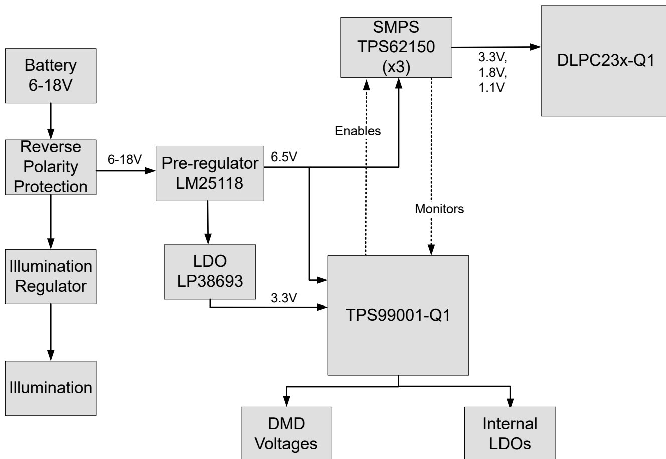
Figure 8-1. Headlight Power Supply Architecture
