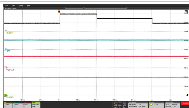
Figure 5-18. Transient Overvoltage
