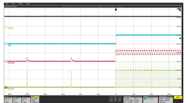
Figure 5-31. LED Short-Circuit Recovery in Fail-Safe Mode
