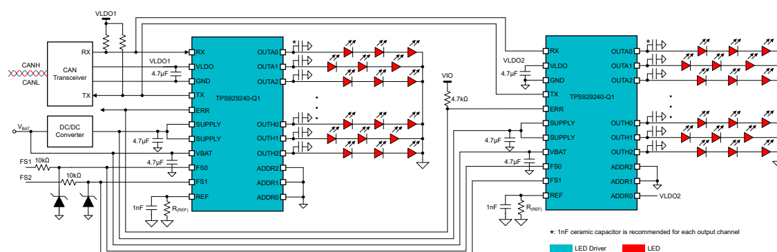
Figure 7-2. Typical Application Schematic
