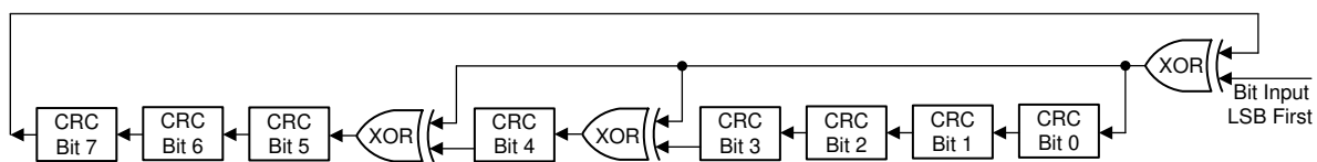
Figure 8-7. CRC Algorithm Diagram
