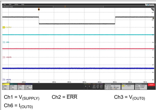
Figure 7-14. Transient Undervoltage
