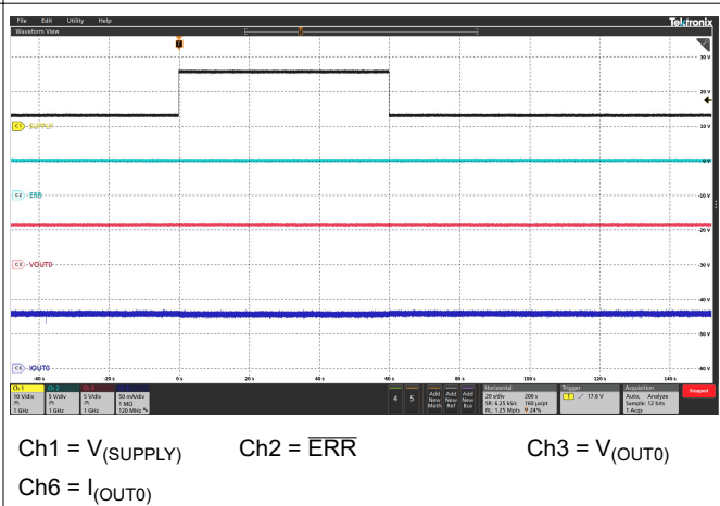
Figure 7-16. Jump Start
