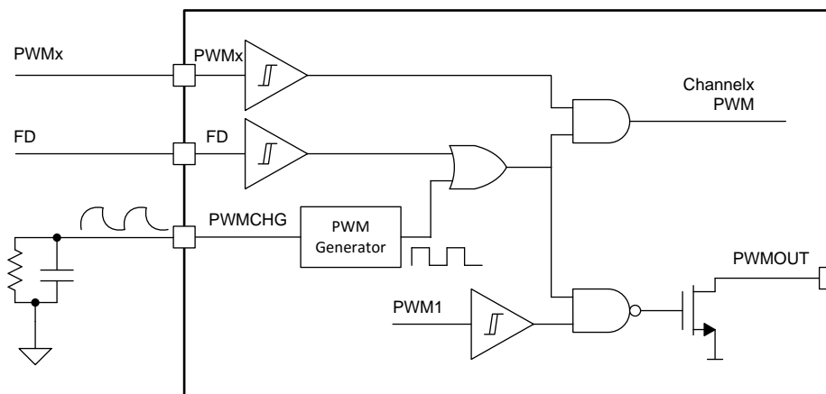
Figure 25. PWM Dimming Internal Block Diagram
