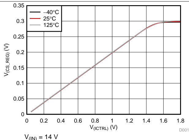
Figure 4. Current-Sense Voltage vs CTRL Input Voltage
