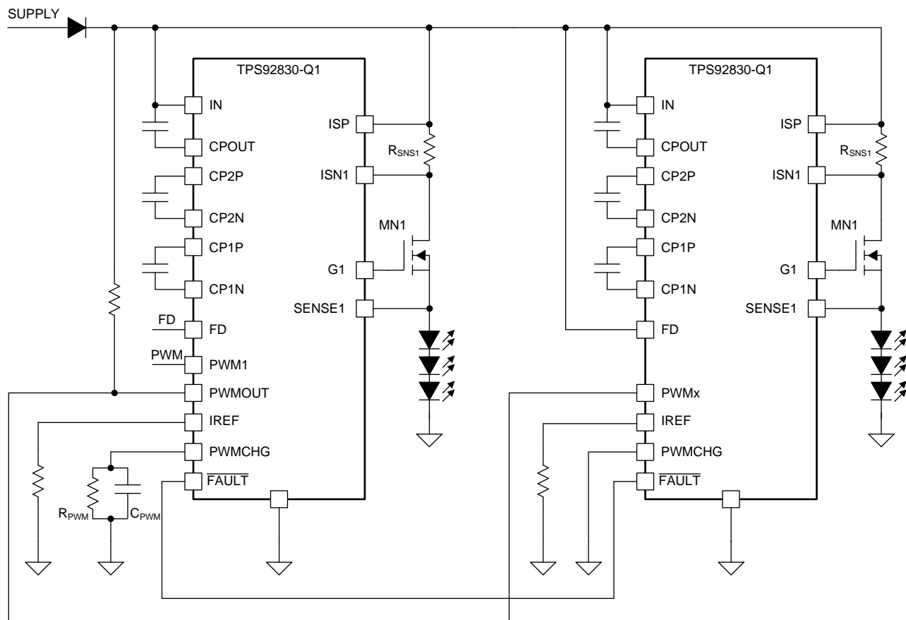
Figure 33. PWM Generator Master-Slave Configuration
