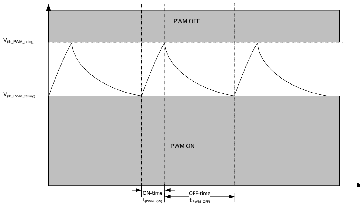
Figure 24. PWM Dimming Profile
