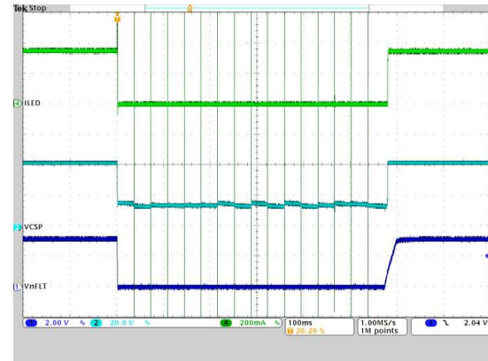
Figure 51. LED Short-Circuit Fault
