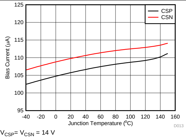
Figure 14. CSP/CSN Input Bias Current vs Junction Temperature
