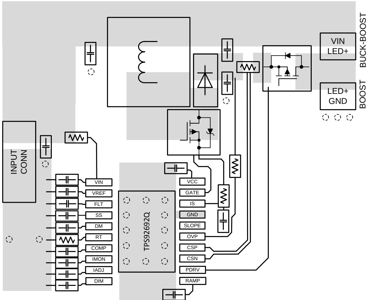
Figure 59. Layout Recommendation
