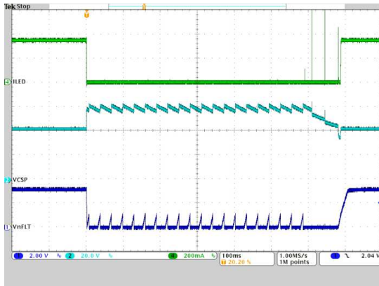
Figure 50. LED Open-Circuit Fault
