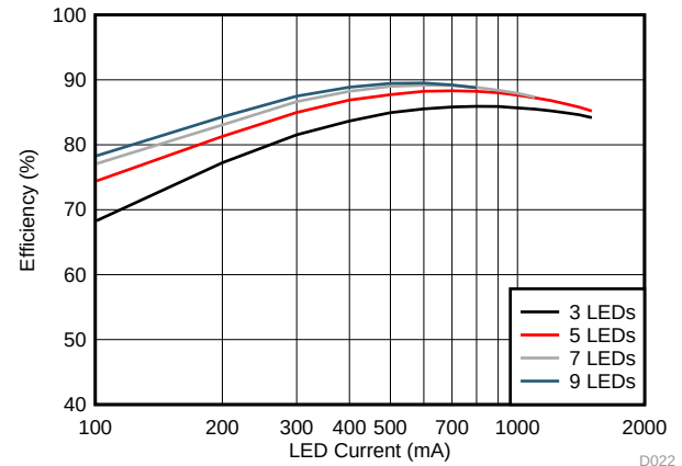
Figure 56. Efficiency
