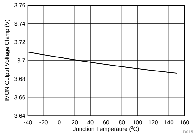
Figure 16. V_{IMON(CLIP)} vs Junction Temperature
