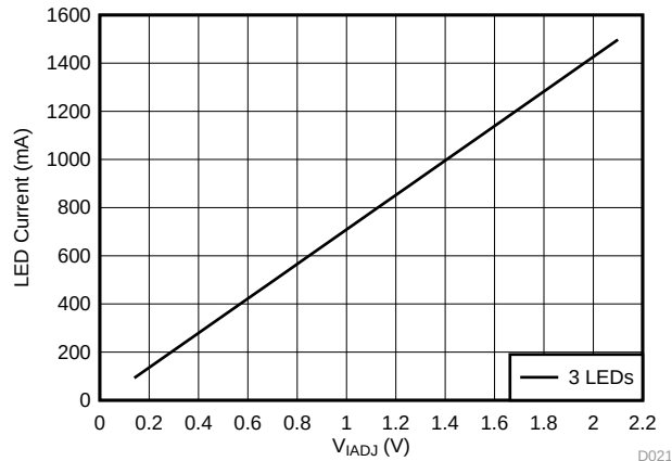
Figure 55. LED Current vs IADJ Voltage
