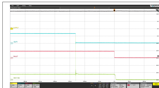
Figure 6-13. LED Short-Circuit Protection
