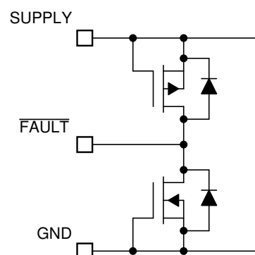
Figure 7-17. FAULT Pin
