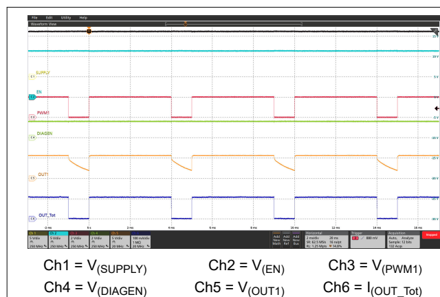
Figure 8-5. PWM Dimming 80% Dutycycle at 200 Hz
