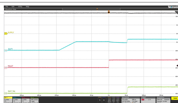
Figure 6-14. LED Short-Circuit Protection Recovery
