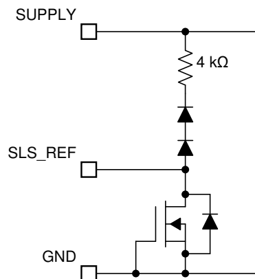
Figure 7-23. SLS_REF Pin
