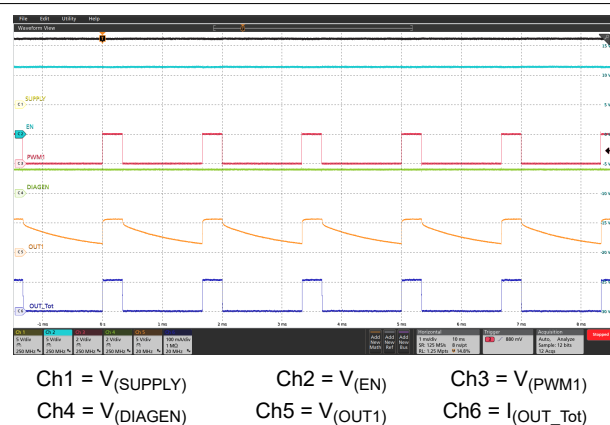
Figure 8-6. PWM Dimming 20% Dutycycle at 600 Hz
