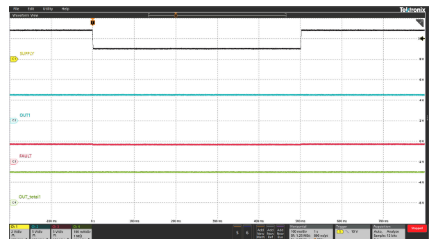
Figure 5-16. LED Short-Circuit Protection
