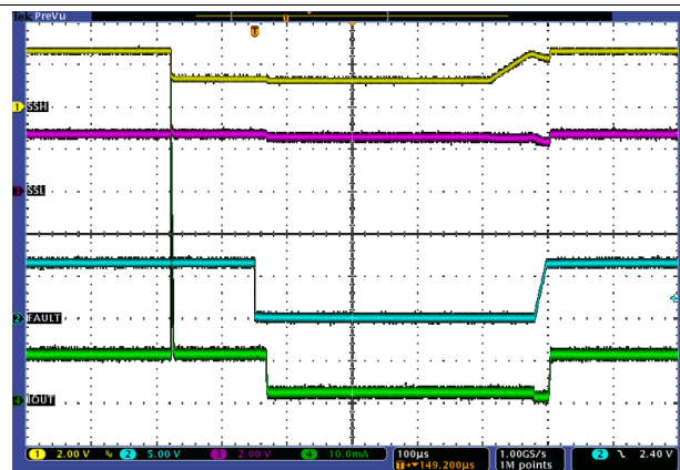
Ch. 1 = V_{(SSH)} Ch. 2 = FAULT Ch. 3 = V_{(SSL)} Ch. 4 = I_{(OUT)}
