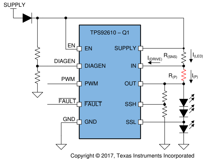
Figure 25. Heat Sharing With a Parallel Resistor
