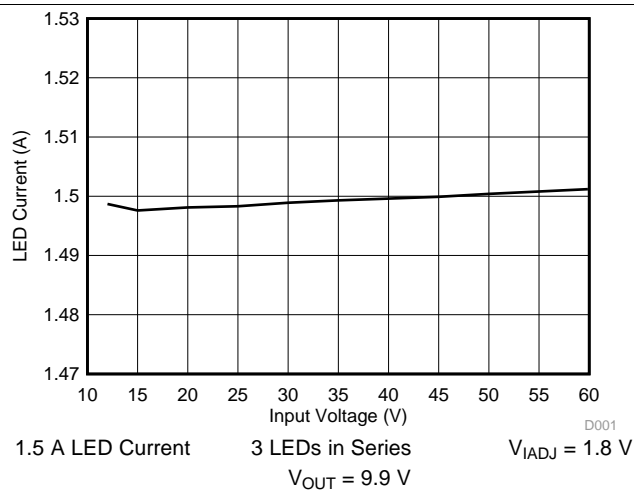
Figure 2. Line Regulation
