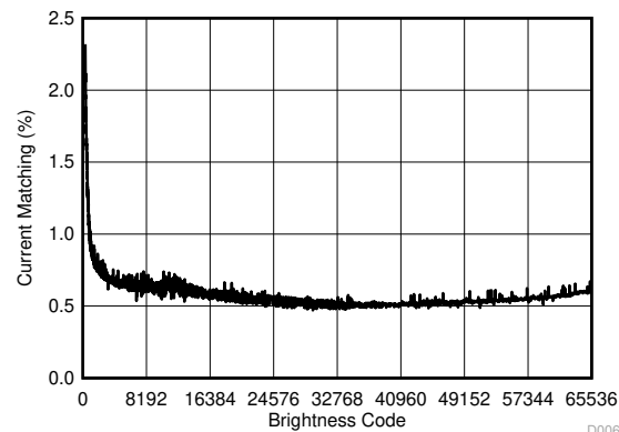
Figure 6-7. Current Matching
