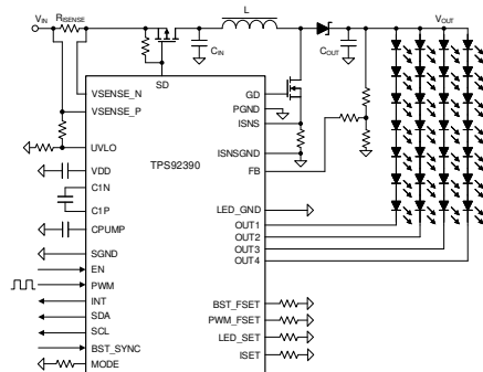
Simplified Schematic
