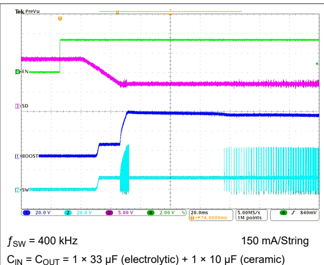
Figure 8-4. Typical Start-Up
