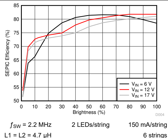
Figure 6-5. SEPIC Efficiency
