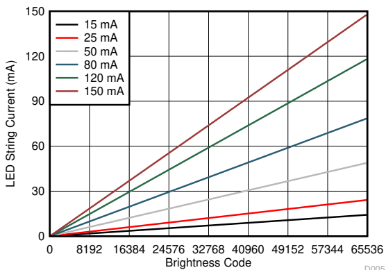
Figure 6-6. Current Linearity
