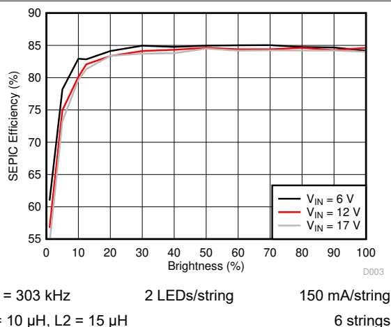
Figure 6-4. SEPIC Efficiency
