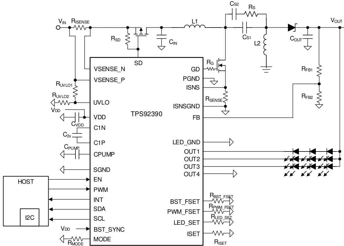
Figure 8-6. SEPIC Mode with Three LEDs in Series
