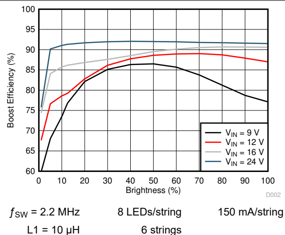
Figure 6-3. Boost Efficiency
