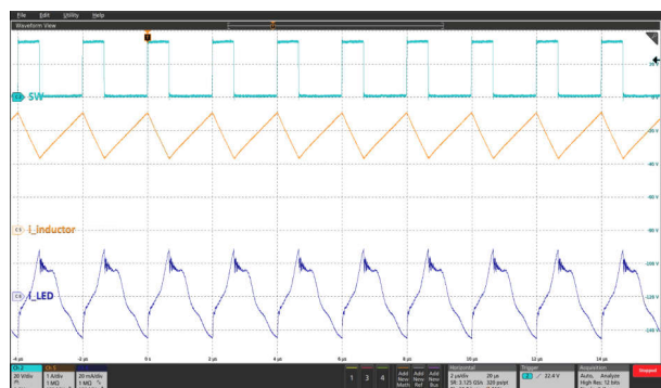
Figure 8-2. LED Current Ripple at PWM_{ADIM} = 100\% , 1kHz and F_{SW} = 500kHz
