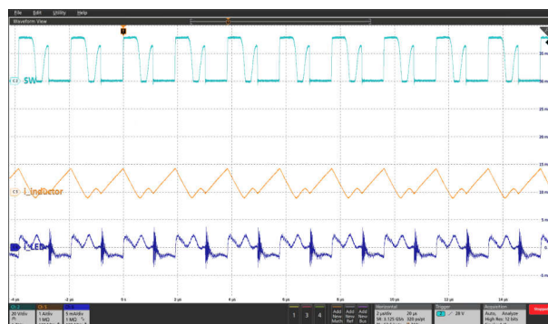
Figure 8-3. LED Current Ripple at PWM_{ADIM} = 10\% , 1kHz and F_{SW} = 500kHz
