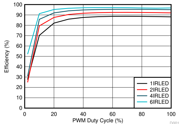
Figure 6-16. Efficiency at 1.5-A Output Current, 4.7-μH Inductor, 12-V Input Voltage
