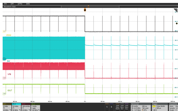
Black: DIM, Blue: SW, Red: FB, Green: LED Current
