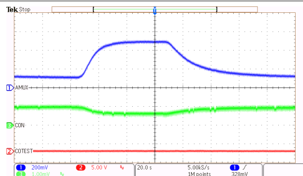
Figure 9-8. Carbon Monoxide Amplifier Waveforms with Calibration Gas
