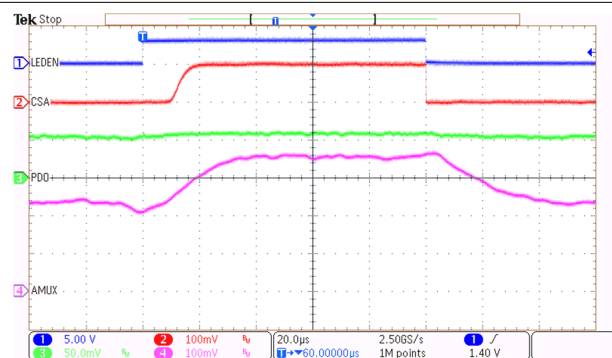
Figure 9-6. LED Driver and Photo Amplifier Waveforms
