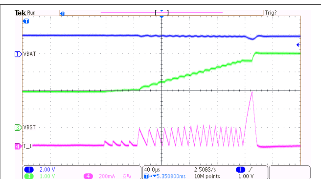
Figure 9-3. Boost Soft-Start
