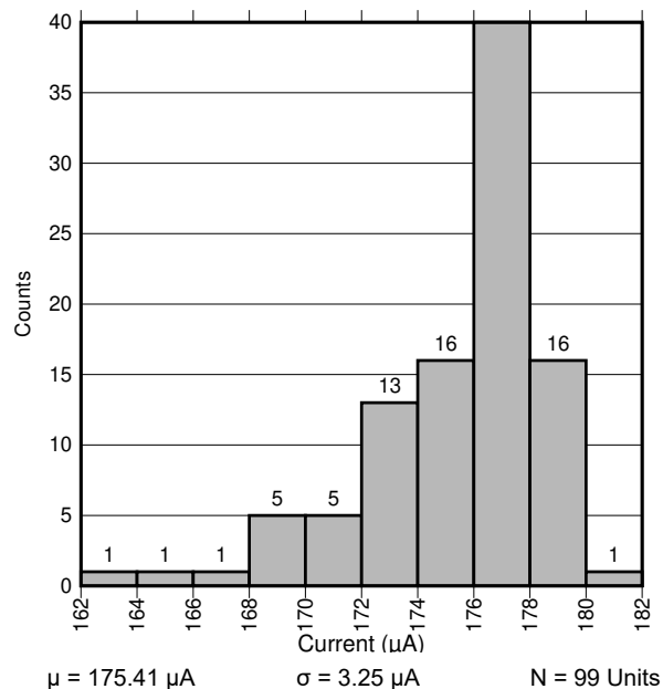
Figure 6-1. 8 MHz Oscillator Current
