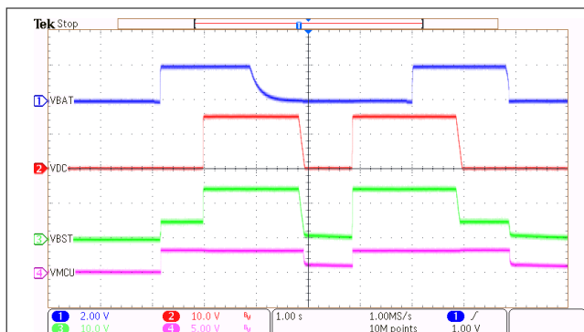
Figure 9-4. 15V AC/DC Supply with Battery Backup Handoff
