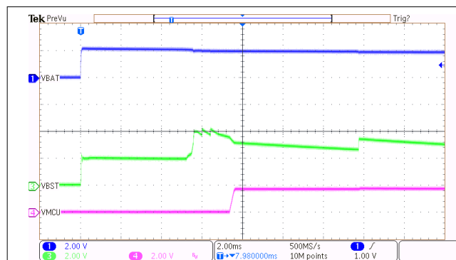
Figure 9-2. Power-up Waveforms
