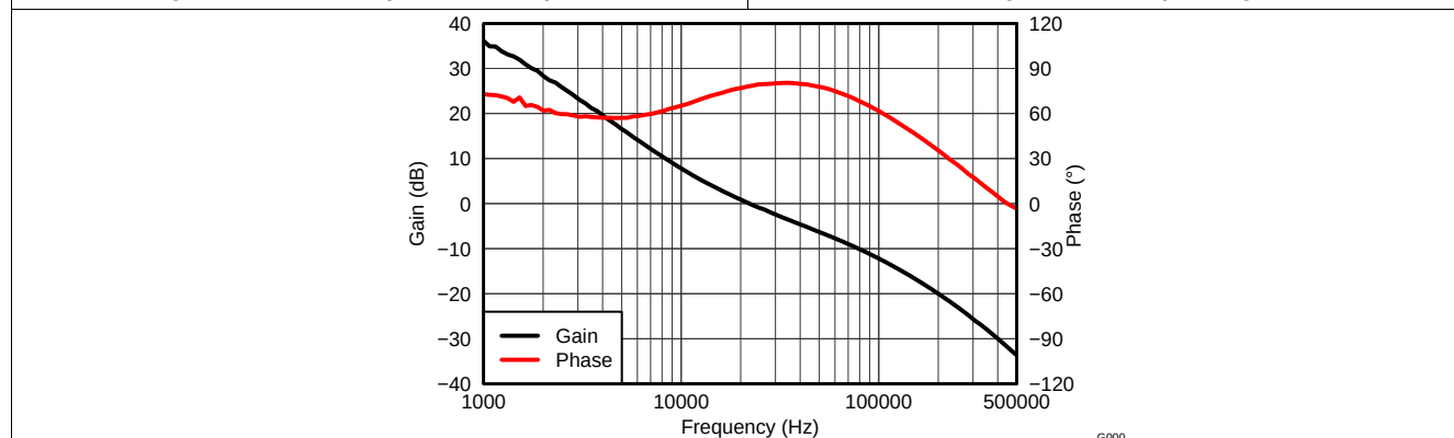
Figure 10. VOUT = 1.8 V, IOUT = 6 A, COUT1 = 47 \mu F ceramic, COUT2 = 100 \mu F POSCAP, fSW = 1 MHz
