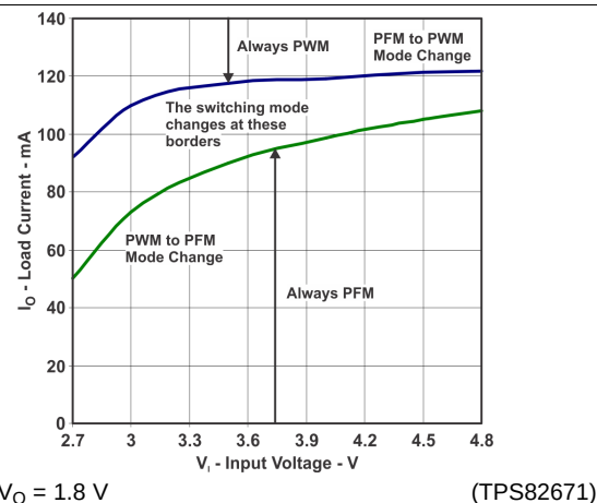
Figure 39. PFM/PWM Boundaries
