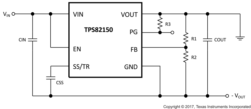
Figure 30. Inverting Power Supply Schematic
