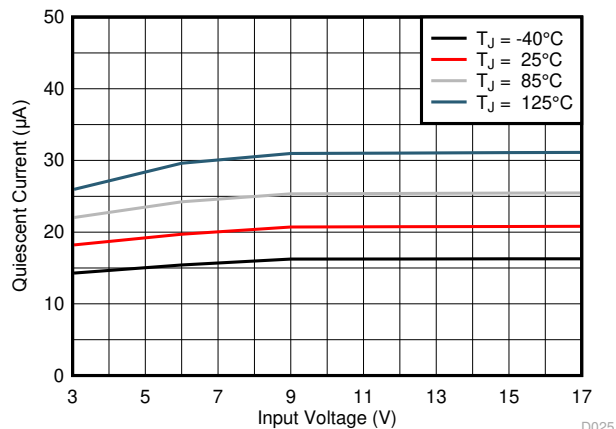
Figure 6-2. Quiescent Current
