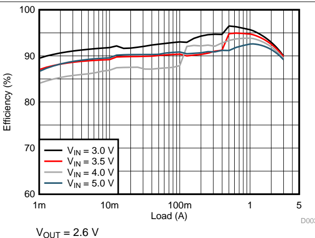
Figure 10. Efficiency
