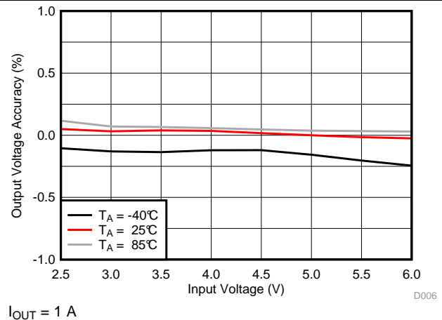
Figure 17. Line Regulation
