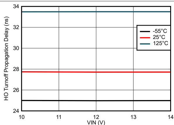
Figure 7-7. HO Turnoff Propagation Delay vs VIN Voltage (IIM)
