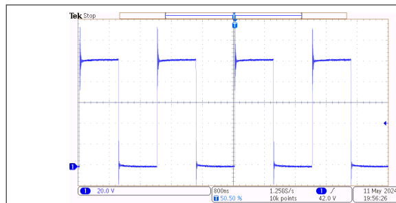
Figure 9-2. 100V, 500kHz Switch Node Signal From TPS7H6005EVM
