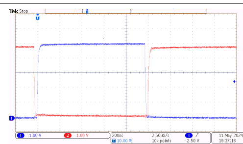
Figure 9-3. 500kHz HO (blue) and LO (red) Gate Driver Outputs in PWM Mode From TPS7H6005EVM
