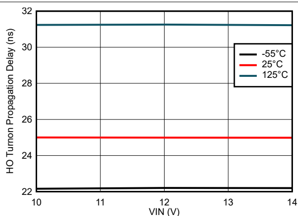
Figure 7-8. HO Turnon Propagation Delay vs VIN Voltage (IIM)
