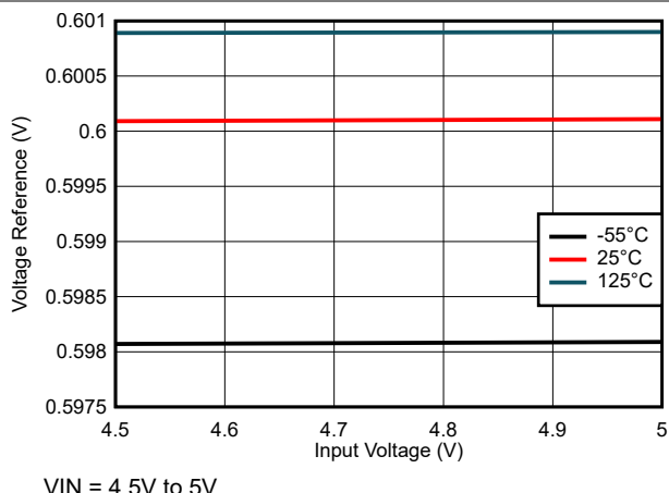
Figure 6-20. Internal Voltage Reference vs Input Voltage
