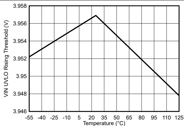
Figure 6-4. VIN UVLO Rising Threshold vs Temperature
