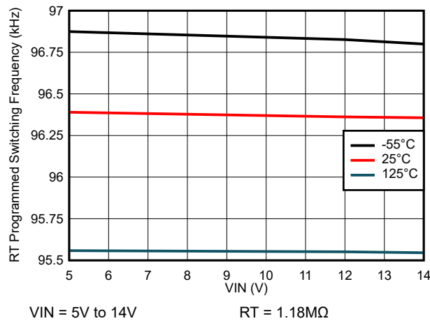
Figure 6-13. Switching Frequency vs Input Voltage
