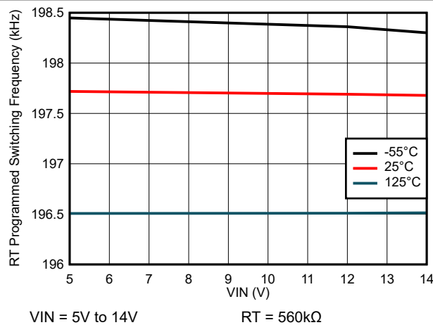
Figure 6-15. Switching Frequency vs Input Voltage
