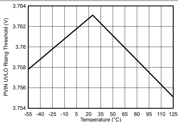
Figure 6-6. PVIN UVLO Rising Threshold vs Temperature
