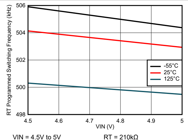
Figure 6-16. Switching Frequency vs Input Voltage
