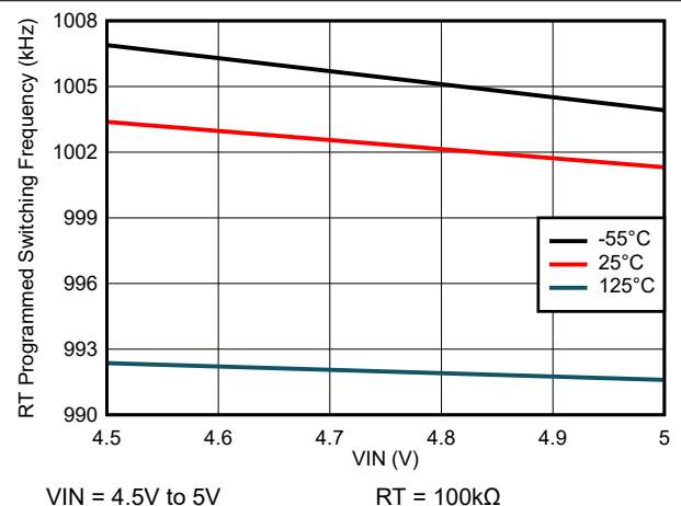
Figure 6-18. Switching Frequency vs Input Voltage
