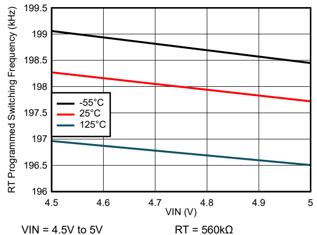
Figure 6-14. Switching Frequency vs Input Voltage
