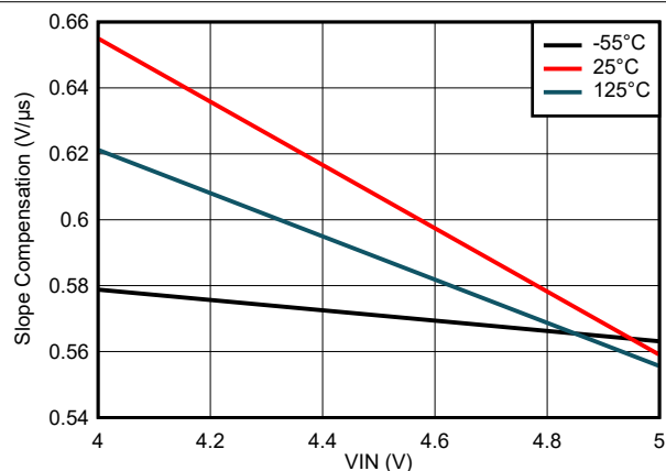
Figure 7-69. Slope Compensation Variation
