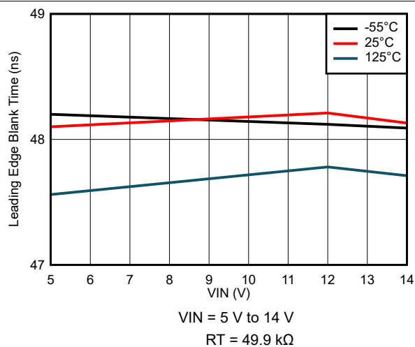
Figure 7-36. Leading Edge Blank Time Variation
