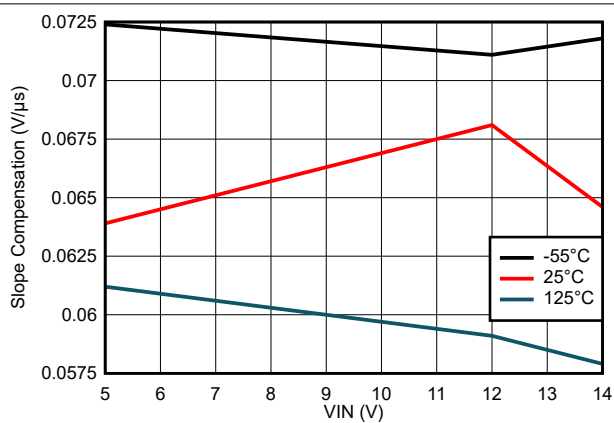
Figure 7-68. Slope Compensation Variation
