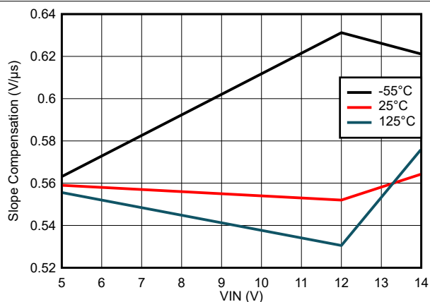
Figure 7-70. Slope Compensation Variation
