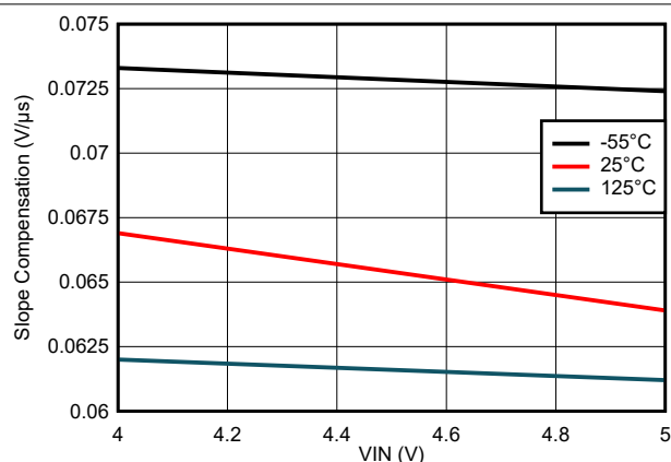
Figure 7-67. Slope Compensation Variation
