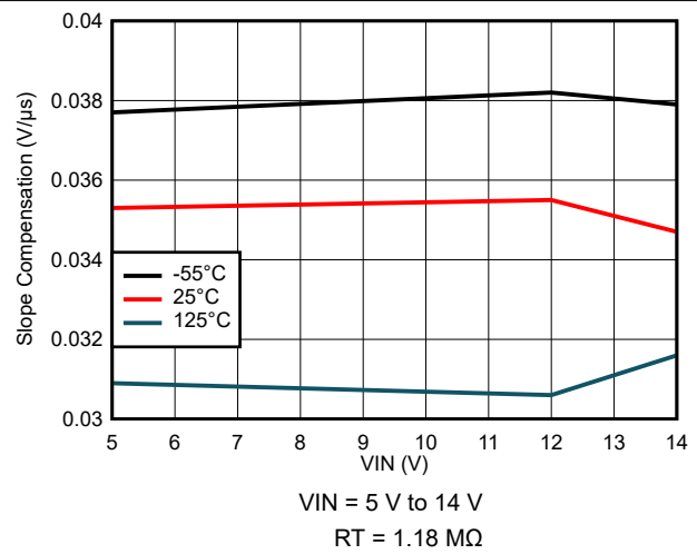
Figure 7-66. Slope Compensation Variation
