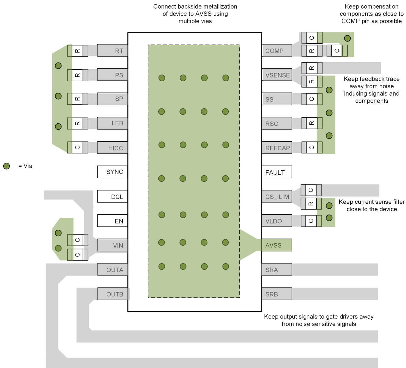
Figure 9-4. PCB Layout Example for CFP Package
