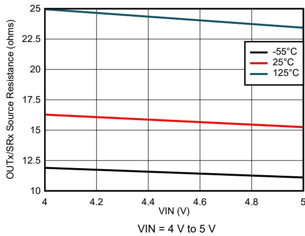
Figure 7-61. Output Source Resistance Variation
