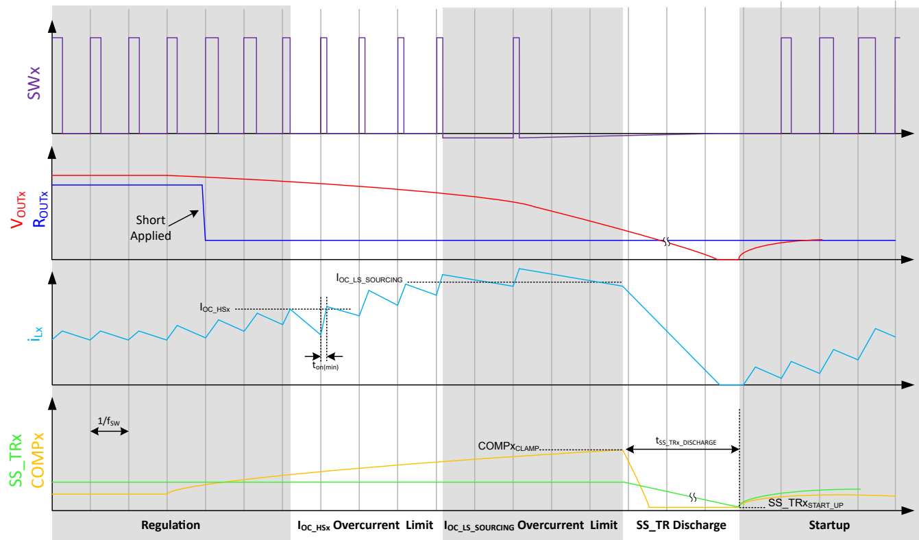
Figure 8-15. COMPx Clamp Shutdown (COMPx_CLAMP)
