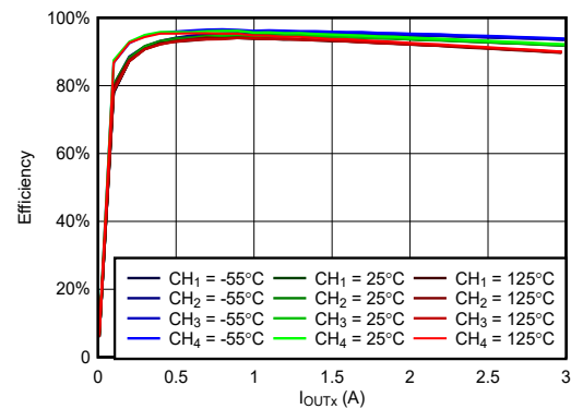
Figure 6-18. Efficiency vs Load at VIN = 7V, VOUTx = 3.3V, fSW = 100kHz
