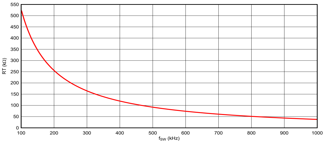
Figure 8-7. Nominal RT vs Switching Frequency
