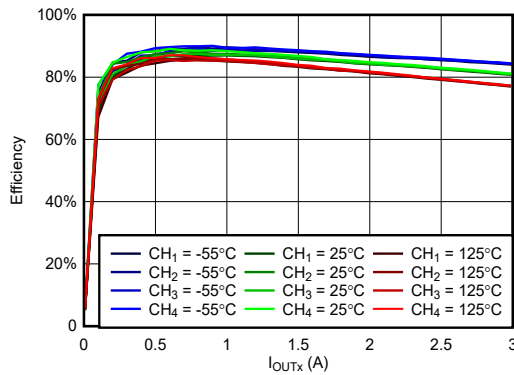
Figure 6-27. Efficiency vs Load at VIN = 5V, VOUTx = 1.2V, fSW = 500kHz
