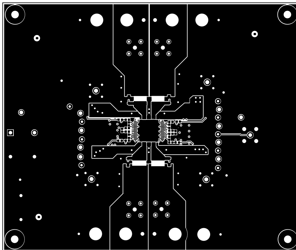
Figure 9-16. PCB Layout Example-Top Layer
