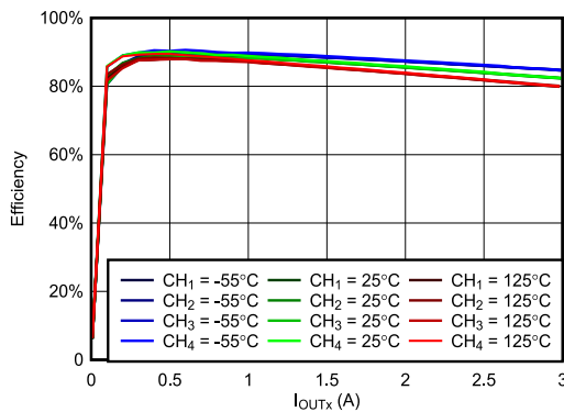
Figure 6-41. Efficiency vs Load at VIN = 3.3V, VOUTx = 1.8V, fSW = 1MHz
