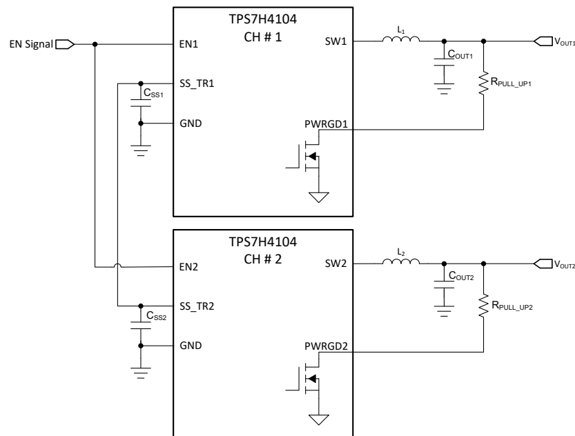
Figure 8-11. Ratiometric Start-Up Sequence
