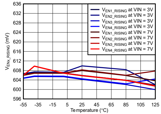
Figure 6-58. EN Rising Threshold vs Temperature
