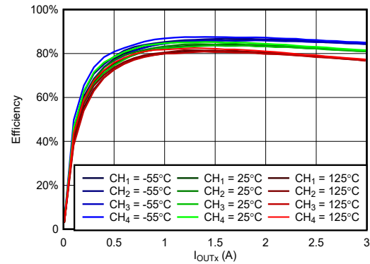
Figure 6-14. Efficiency vs Load at VIN = 7V, VOUTx = 1.2V, fSW = 100kHz
