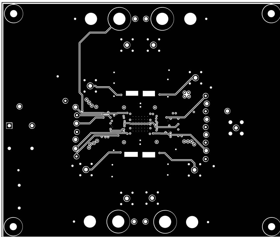
Figure 9-18. PCB Layout Example-Internal Layer 2
