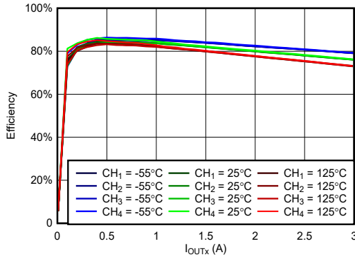
Figure 6-39. Efficiency vs Load at VIN = 3.3V, VOUTx = 1.2V, fSW = 1MHz
