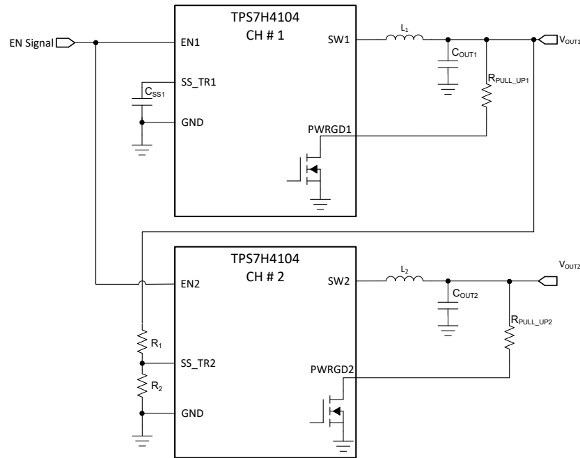
Figure 8-12. Ratiometric and Simultaneous Start-Up Sequence
