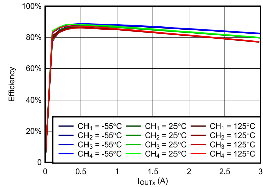
Figure 6-40. Efficiency vs Load at VIN = 3.3V, VOUTx = 1.5V, fSW = 1MHz
