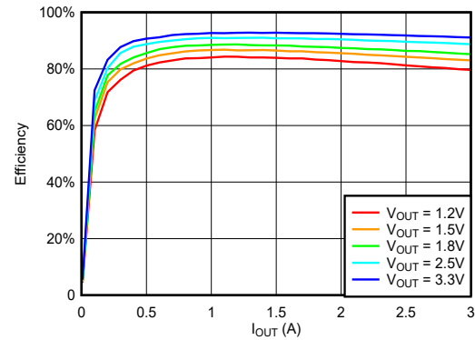
Figure 6-38. Efficiency vs Load at VIN = 7V, Across VOUT at fSW = 500kHz for Channel # 1 at 25°C
