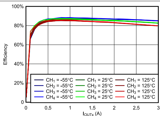
Figure 6-45. Efficiency vs Load at VIN = 5V, VOUTx = 1.8V, fSW = 1MHz
