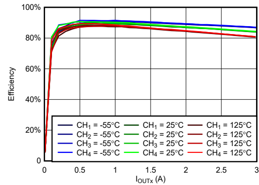
Figure 6-28. Efficiency vs Load at VIN = 5V, VOUTx = 1.5V, fSW = 500kHz
