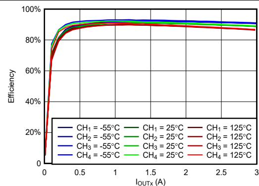
Figure 6-36. Efficiency vs Load at VIN = 7V, VOUTx = 2.5V, fSW = 500kHz
