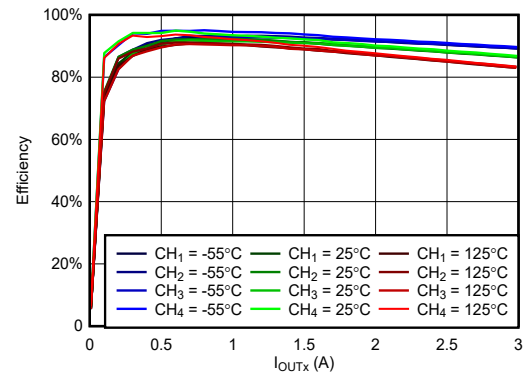
Figure 6-16. Efficiency vs Load at VIN = 7V, VOUTx = 1.8V, fSW = 100kHz
