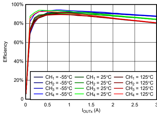
Figure 6-15. Efficiency vs Load at VIN = 7V, VOUTx = 1.5V, fSW = 100kHz
