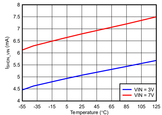
Figure 6-54. VIN Shutdown Current vs Temperature
