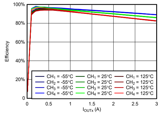
Figure 6-4. Efficiency vs Load at VIN = 3.3V, VOUTx = 1.8V, fSW = 100kHz
