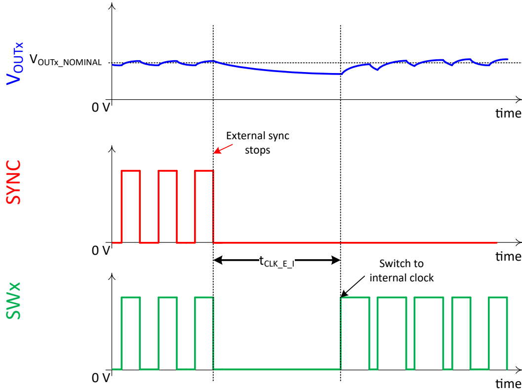
Figure 8-9. External to Internal Clock Transition
