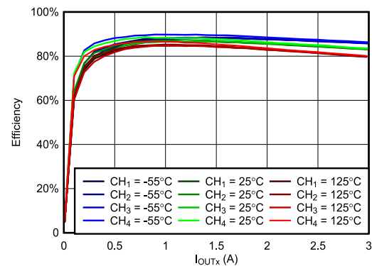
Figure 6-34. Efficiency vs Load at VIN = 7V, VOUTx = 1.5V, fSW = 500kHz
