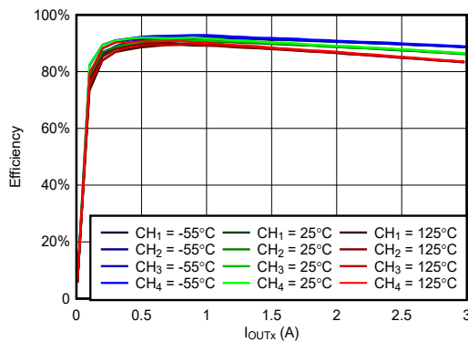
Figure 6-29. Efficiency vs Load at VIN = 5V, VOUTx = 1.8V, fSW = 500kHz
