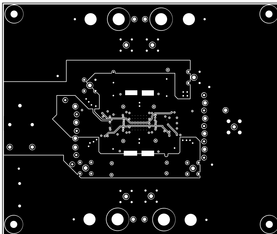
Figure 9-20. PCB Layout Example-Internal Layer 4
