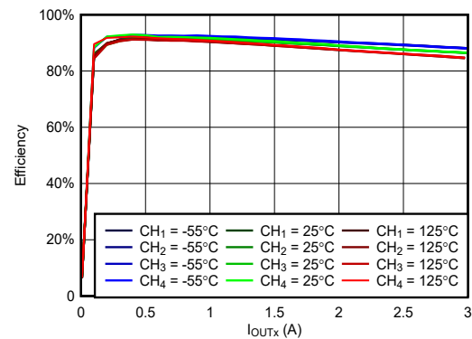
Figure 6-42. Efficiency vs Load at VIN = 3.3V, VOUTx = 2.5V, fSW = 1MHz
