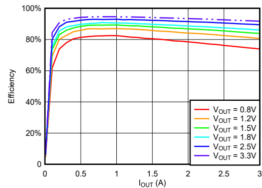
Figure 6-32. Efficiency vs Load at VIN = 5V, Across VOUT at fSW = 500kHz for Channel # 1 at 25°C
