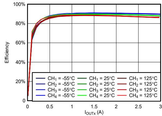
Figure 6-50. Efficiency vs Load at VIN = 7V, VOUTx = 3.3V, fSW = 1MHz
