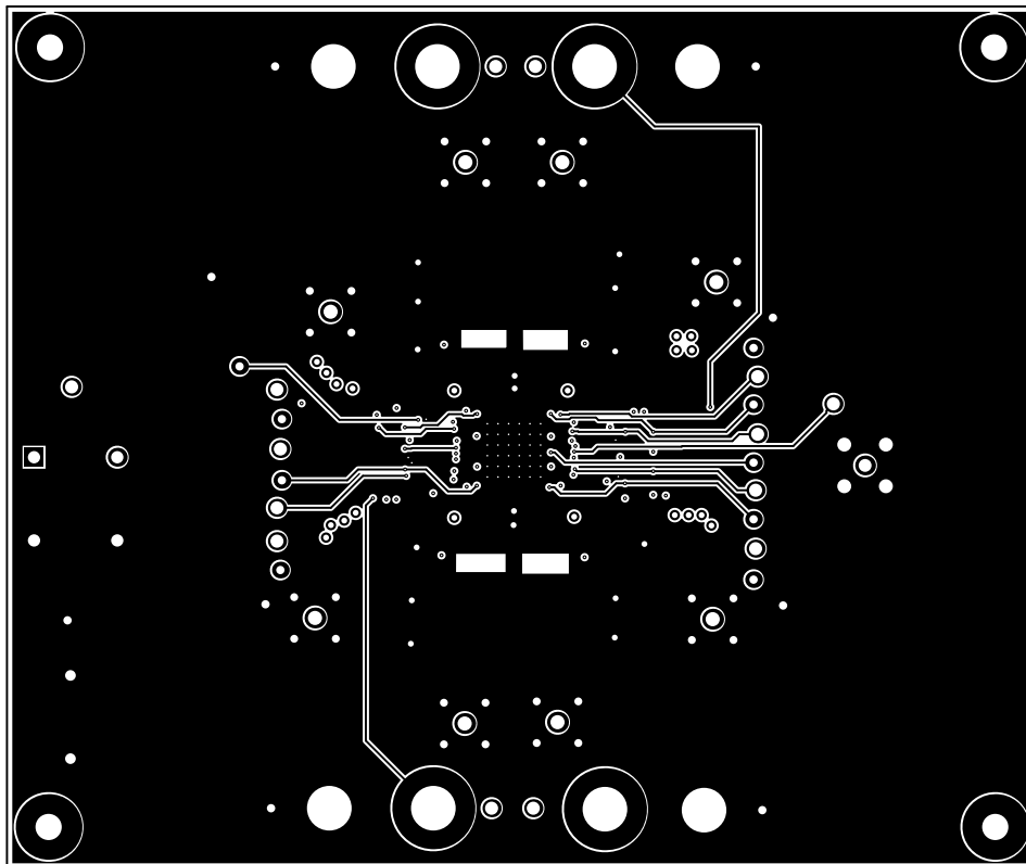
Figure 9-17. PCB Layout Example-Internal Layer 1
