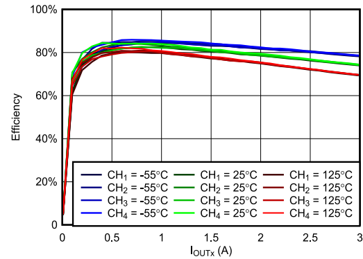
Figure 6-26. Efficiency vs Load at VIN = 5V, VOUTx = 0.8V, fSW = 500kHz
