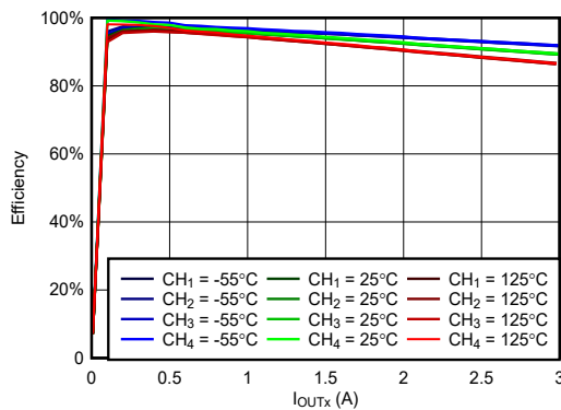
Figure 6-5. Efficiency vs Load at VIN = 3.3V, VOUTx = 2.5V, fSW = 100kHz
