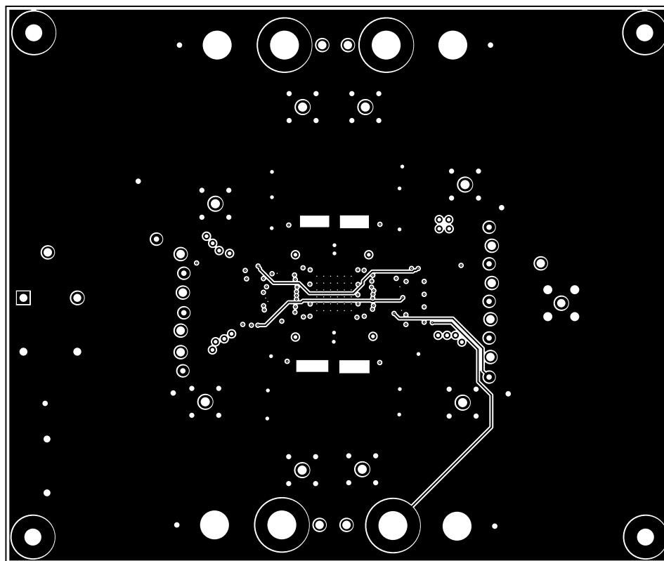
Figure 9-19. PCB Layout Example-Internal Layer 3
