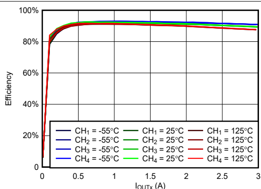
Figure 6-47. Efficiency vs Load at VIN = 5V, VOUTx = 3.3V, fSW = 1MHz
