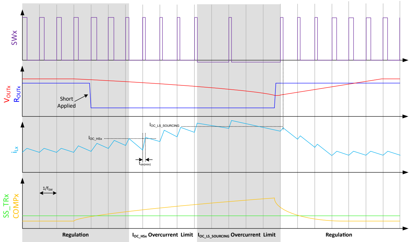
Figure 8-14. Low-Side Sourcing Overcurrent Protection ( I_{OC\_LS\_SOURCINGx} )
