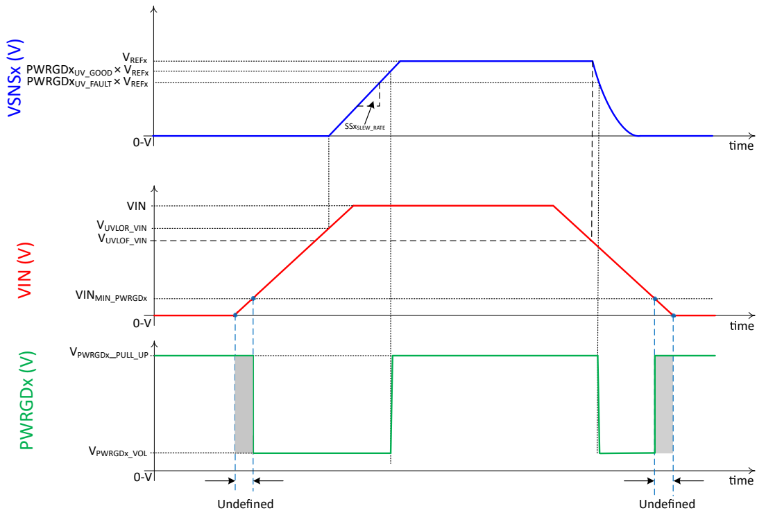
Figure 8-6. PWRGDx in Valid States after V_{IN} > V_{IN\_MIN\_PWRGDx}
