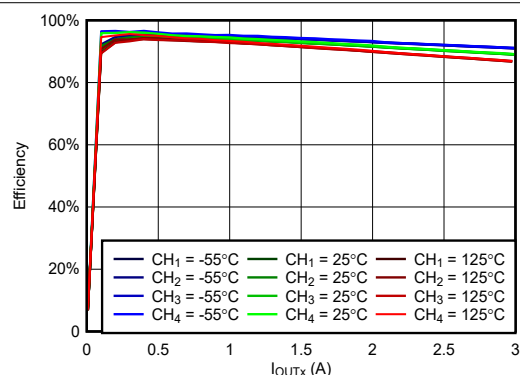
Figure 6-24. Efficiency vs Load at VIN = 3.3V, VOUTX = 2.5V, fSW = 500kHz
