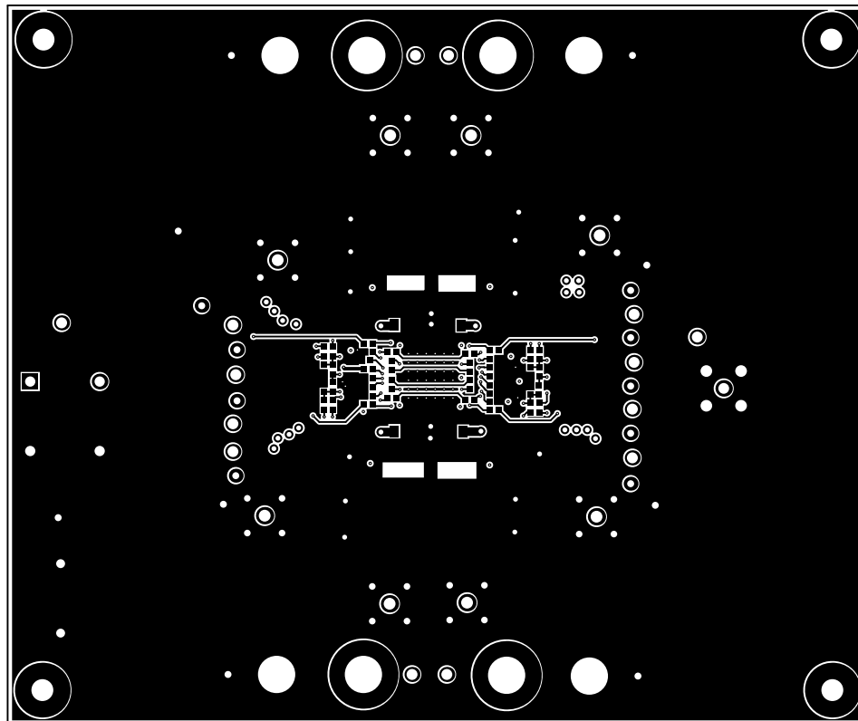
Figure 9-21. PCB Layout Example-Bottom Layer
