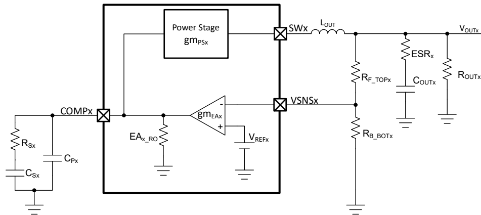
Figure 8-16. Simplified Small Signal Model For Loop Response
