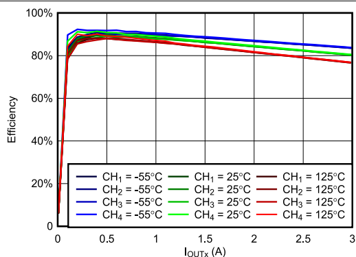
Figure 6-21. Efficiency vs Load at VIN = 3.3V, VOUTX = 1.2V, fSW = 500kHz
