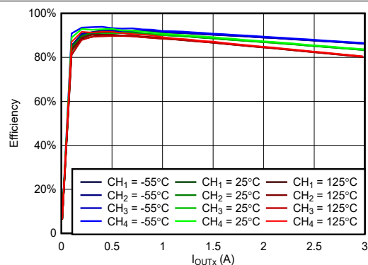
Figure 6-22. Efficiency vs Load at VIN = 3.3V, VOUTX = 1.5V, fSW = 500kHz
