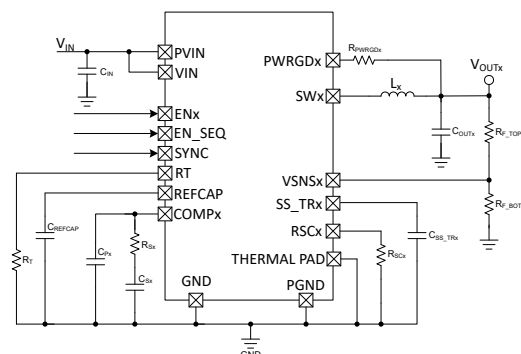
Simplified Schematic
