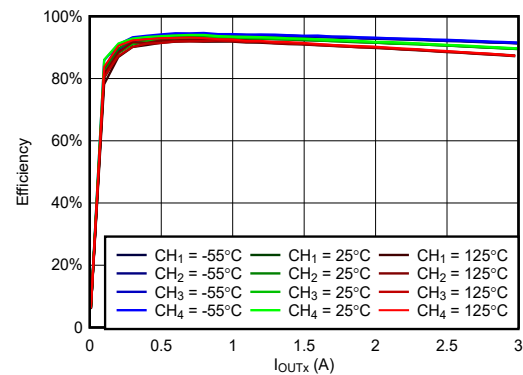
Figure 6-30. Efficiency vs Load at VIN = 5V, VOUTx = 2.5V, fSW = 500kHz
