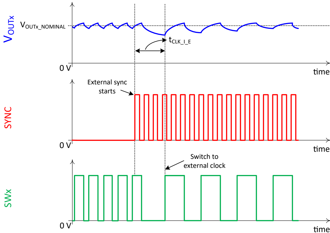
Figure 8-8. Internal to External Clock Transition
