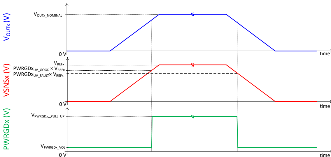
Figure 8-4. PWRGDx Undervoltage (UV) Thresholds
