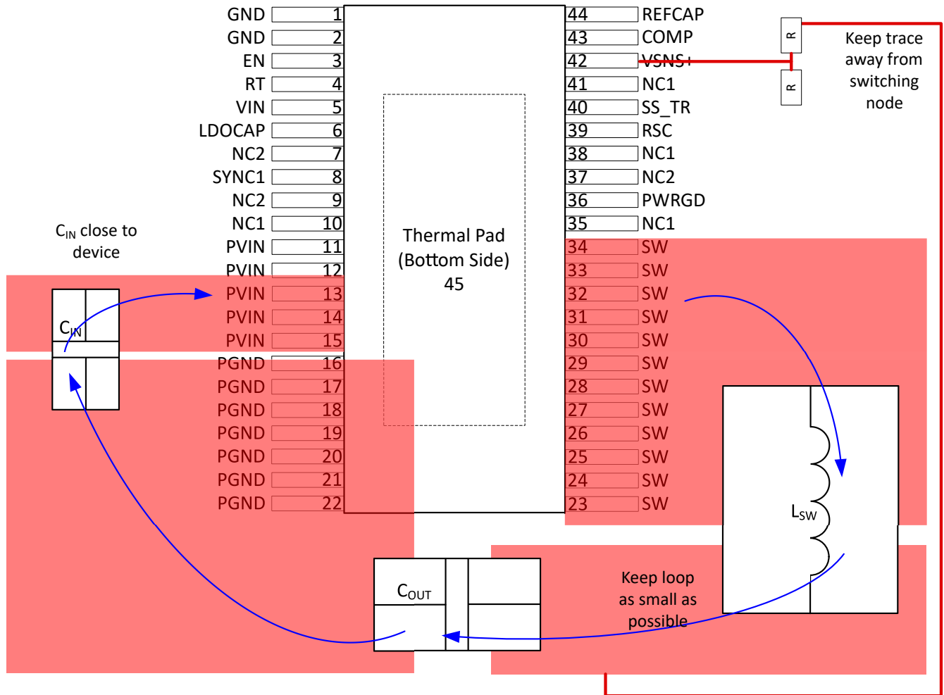
Figure 10-6. Simplified Layout Example
