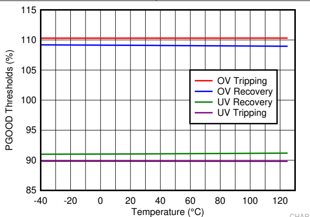
Figure 6-9. PGOOD Thresholds
