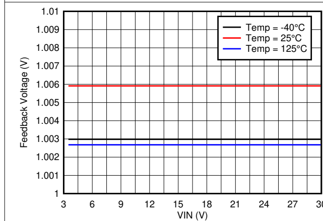
Figure 6-3. Feedback Voltage
