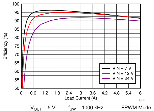
Figure 8-6. TPS7H4010-SEP Efficiency
