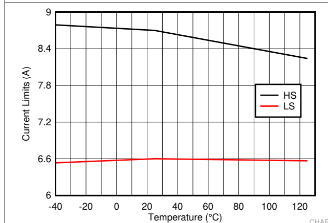
Figure 6-5. TPS7H4010-SEP High-Side and Low-Side Current Limit
