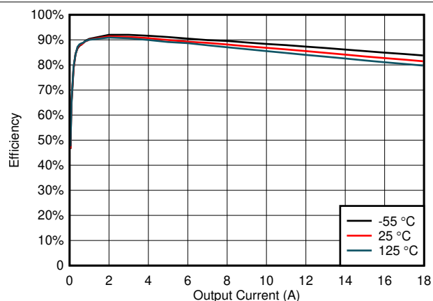
Figure 7-42. Efficiency for VIN = 5 V, VOUT = 2.5 V at 1000-kHz Switching Frequency
