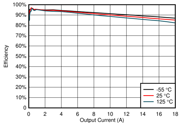
Figure 7-38. Efficiency for VIN = 3 V, VOUT = 2.5 V at 1000-kHz Switching Frequency
