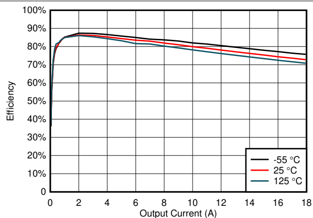
Figure 7-40. Efficiency for VIN = 5 V, VOUT = 1.5 V at 1000-kHz Switching Frequency
