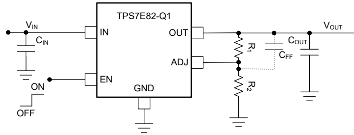
Figure 7-6. TPS7E82 Adjustable LDO Regulator Programming
