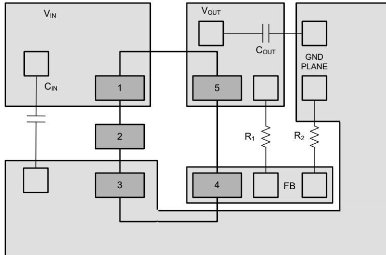
Figure 7-8. Example Layout for TPS7E82 (Without EN) DBV Package
