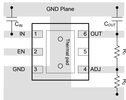
Figure 7-9. Example Layout for TPS7E82 DRV Package
