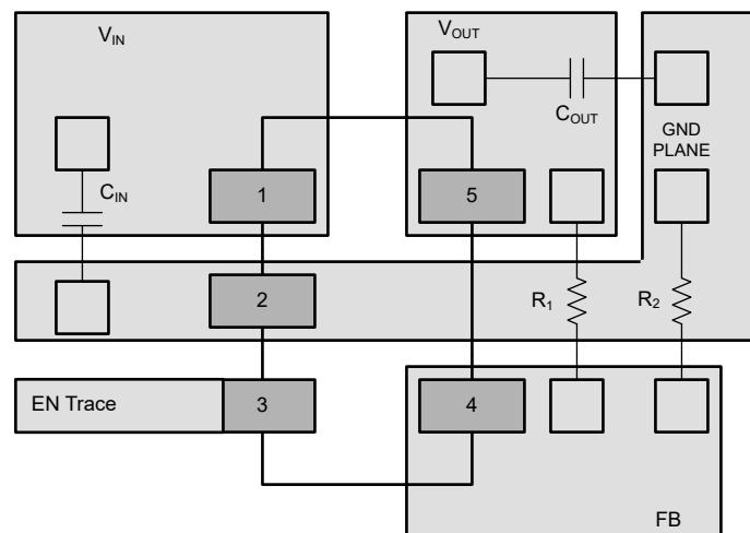
Figure 7-7. Example Layout for TPS7E82 (With EN) DBV Package
