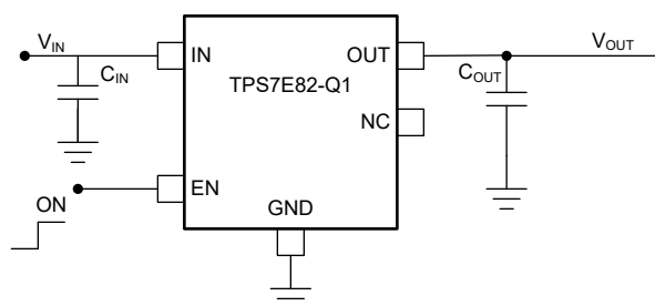
Figure 7-5. TPS7E82 Typical Application Circuit (Fixed-Voltage Version)
