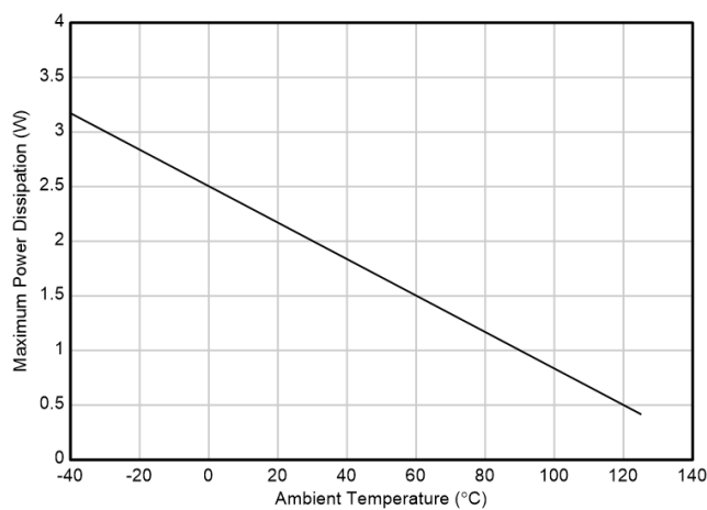
Figure 7-4. TPS7E82 (DGN) Allowable Power Dissipation
