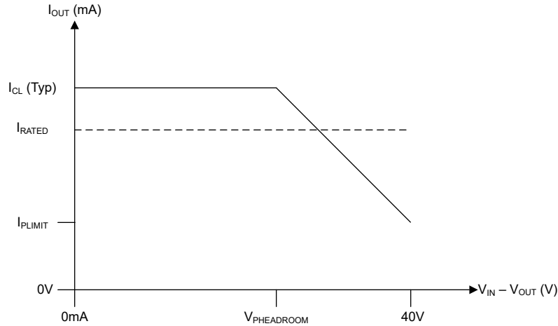
Figure 6-6. Power Limiting
