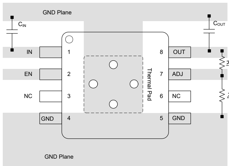
Figure 7-10. Example Layout for TPS7E82 DGN Package
