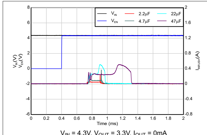
Figure 7-7. Inrush Current vs C_{OUT}
