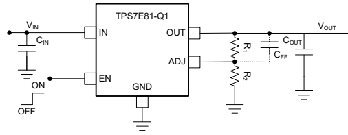
Figure 3-1. Typical Application
