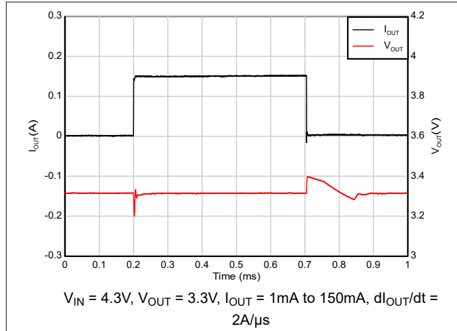
Figure 5-43. Load Transient (1mA to 150mA)
