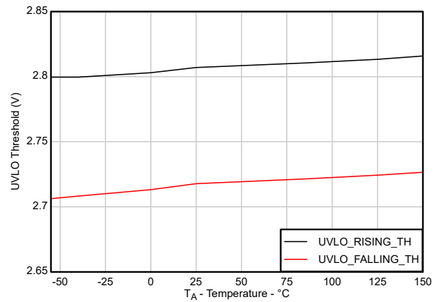
Figure 5-14. UVLO Threshold ( V_{UVLO+}/V_{UVLO-} ) vs Temperature
