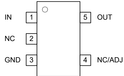
Figure 4-4. DBV Package, [A-version, w/o EN] (Fixed/ADJ), 5-Pin SOT-23 (Top View)
