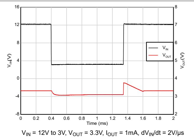
Figure 5-46. Dropout Recovery (12V to 3V)
