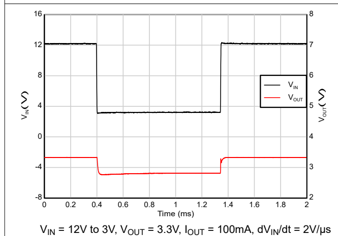
Figure 5-47. Dropout Recovery (12V to 3V)
