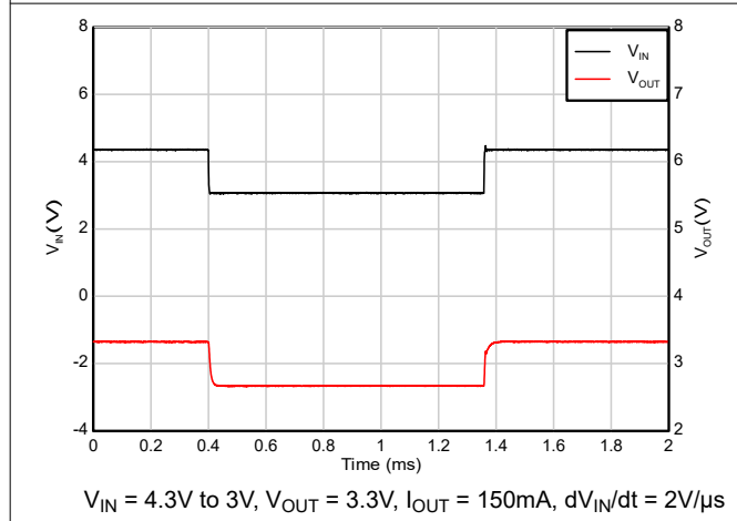
Figure 5-45. Dropout Recovery (4.3V to 3V)
