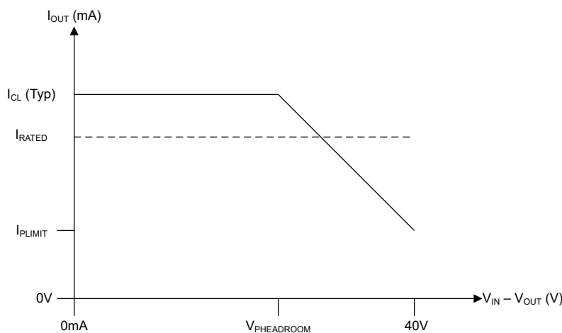
Figure 6-6. Power Limiting
