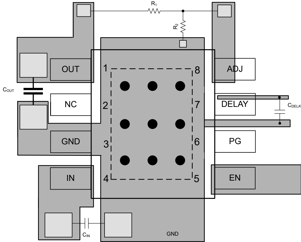
Figure 7-18. Example layout for TPS7E67-Q1 DDA Package
