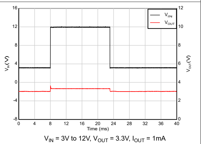
Figure 5-50. Cold-crank Recovery
