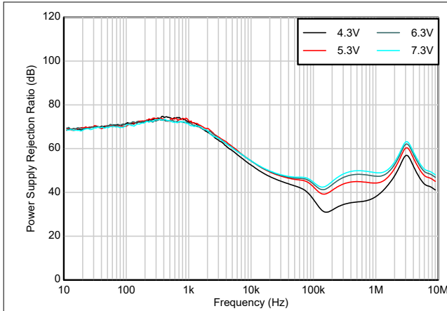
Figure 5-23. PSRR vs V_{IN}
