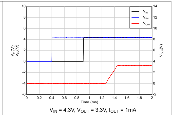
Figure 5-38. Start-up with sequencing ( V_{IN} after EN)
