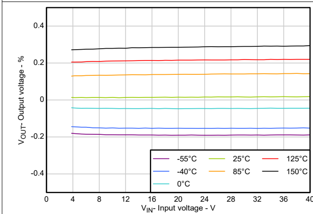
Figure 5-3. V_{OUT} Accuracy vs V_{IN}
