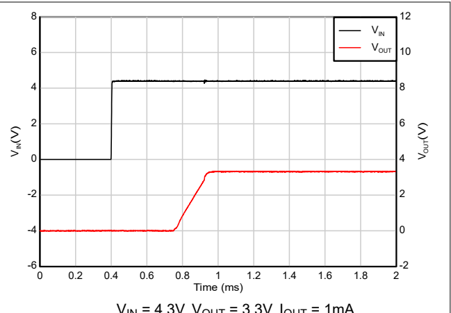
Figure 5-32. Start-up with EN & V_{IN} tied together
