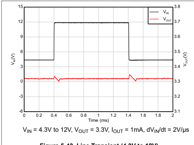
Figure 5-43. Line Transient (4.3V to 12V)
