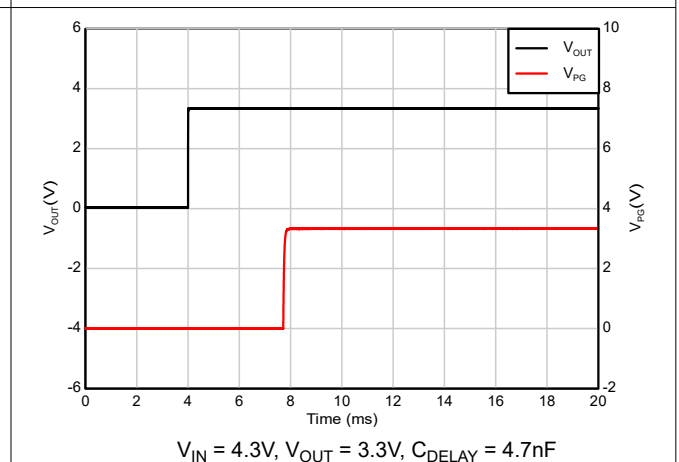
Figure 5-42. PG Delay with C_{DELAY} = 4.7\text{nF}
