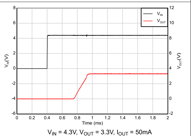
Figure 5-34. Start-up with EN & V_{IN} tied together
