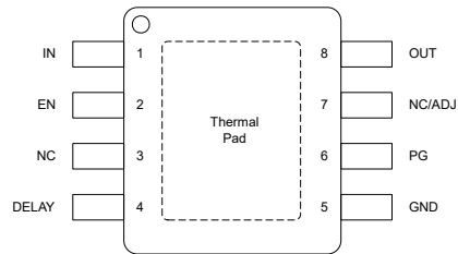
Figure 4-3. DGN Package (Fixed/ADJ), 8-Pin HVSSOP (Top View)
