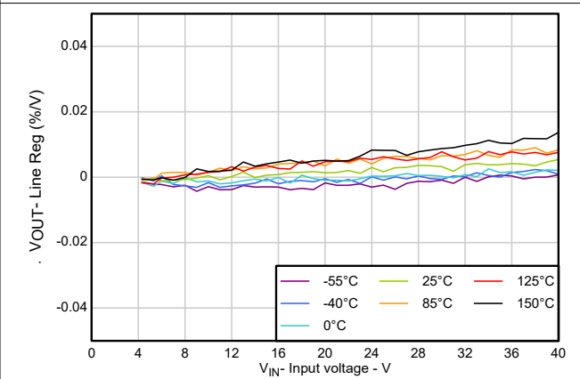
Figure 5-4. Line Regulation
