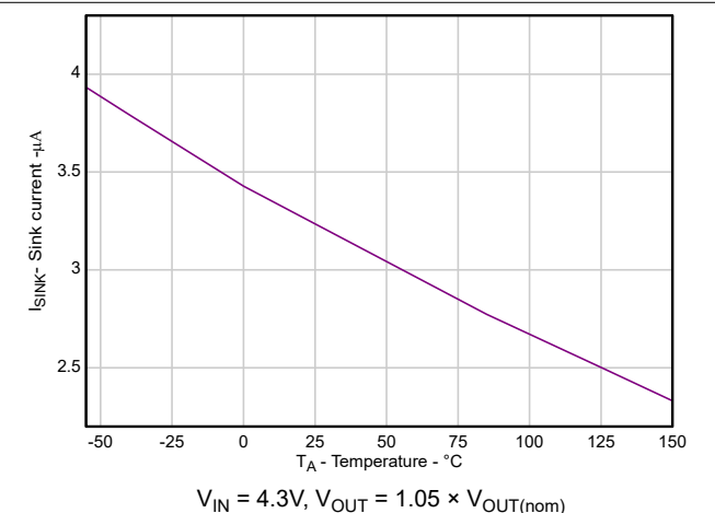
Figure 5-16. Sink Current on Output ( I_{SINK} ) vs Temperature
