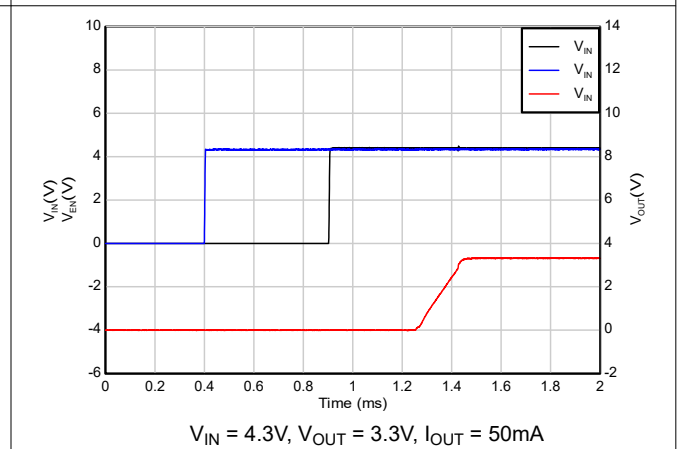
Figure 5-40. Start-up with sequencing ( V_{IN} after EN)
