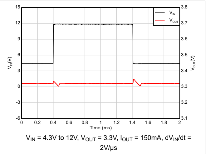
Figure 5-44. Line Transient (4.3V to 12V)
