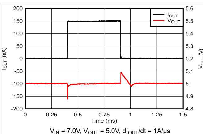
Figure 5-26. Load Transient (1mA to 150mA)
