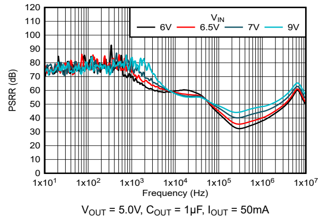
Figure 5-32. PSRR vs Input Supply
