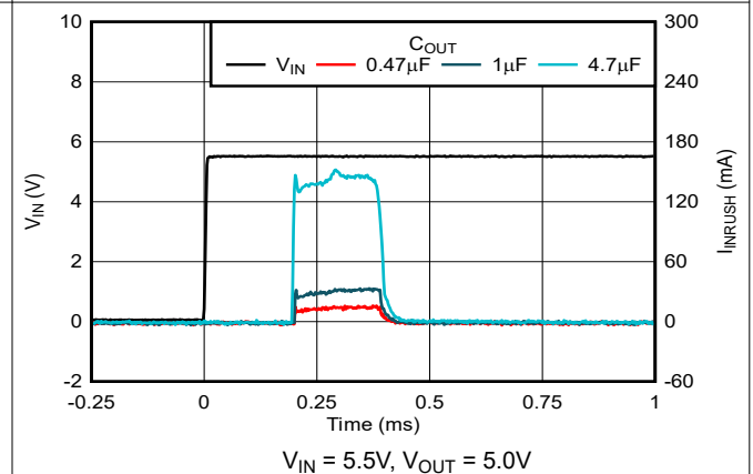
Figure 7-15. Inrush Current vs Output Capacitor
