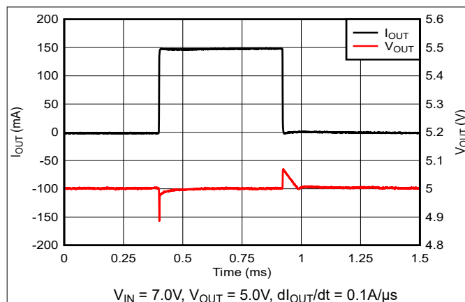
Figure 5-25. Load Transient (1mA to 150mA)
