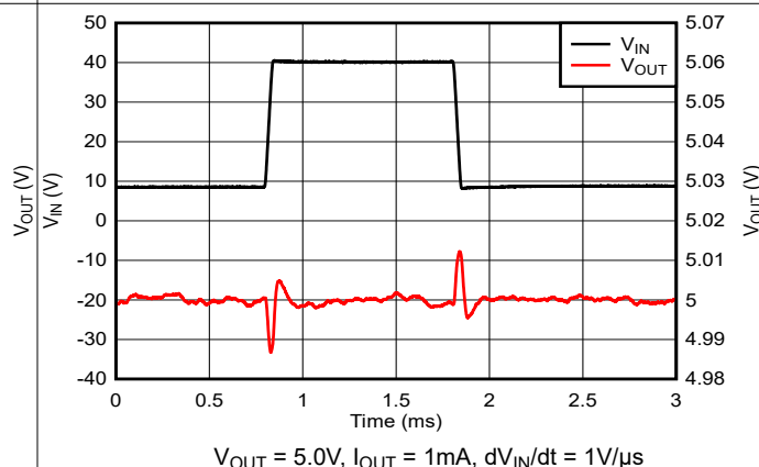
Figure 5-24. V_{IN} Line Transient (8.8V to 40V)
