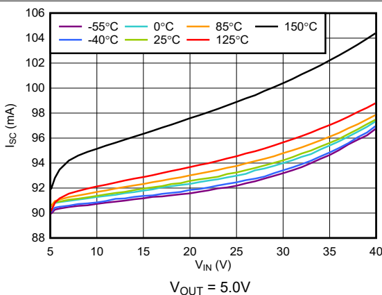
Figure 5-17. Short-Current Limit vs V_{IN}
