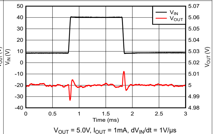
Figure 7-9. V_{IN} Line Transient (8.8V to 40V)
