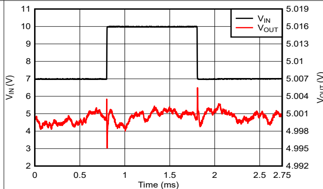
Figure 5-20. V_{IN} Line Transient (7V to 10V)
