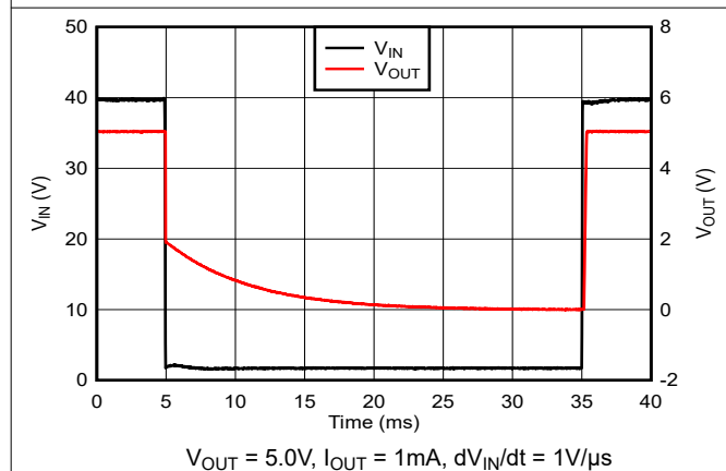
Figure 5-27. Brownout Transient (40V to 1.7V)
