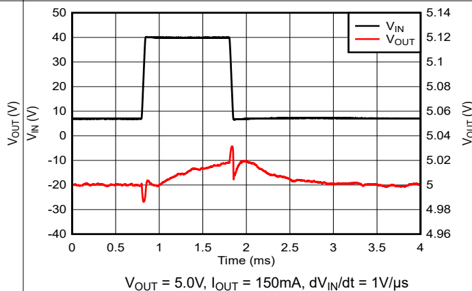
Figure 5-22. V_{IN} Line Transient (7V to 40V)
