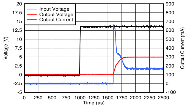
Figure 8-3. Power-Up Waveform
