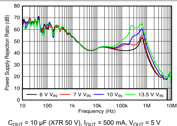
Figure 6-12. PSRR vs Frequency and V_{IN}
