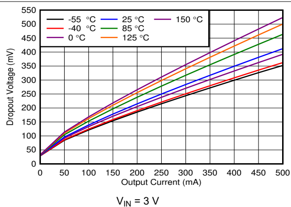
Figure 6-8. Dropout Voltage ( V_{DO} ) vs I_{OUT}
