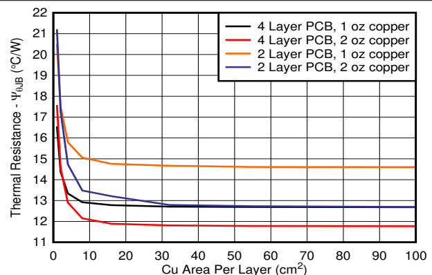
Figure 8-3. \psi_{IB} vs Copper Area (DDA Package)
