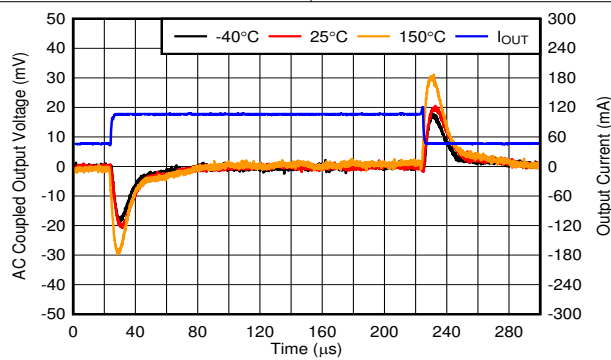
Figure 8-7. Transient Response
