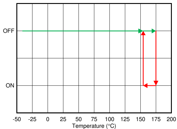
Figure 6-30. Thermal Shutdown
