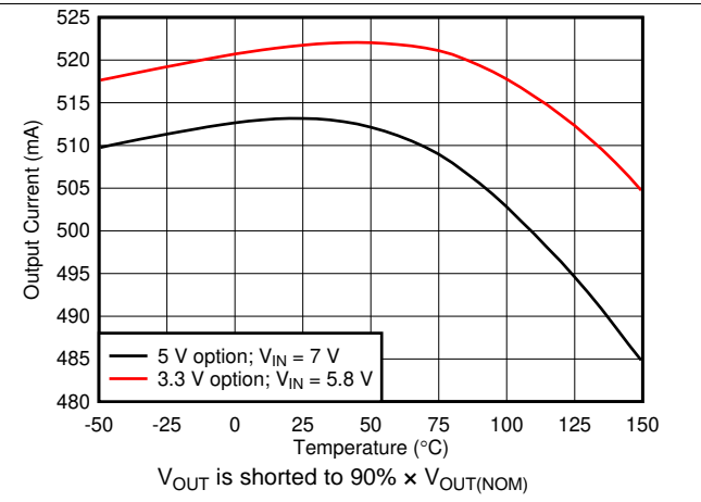
Figure 14. Output Current Limit vs Ambient Temperature
