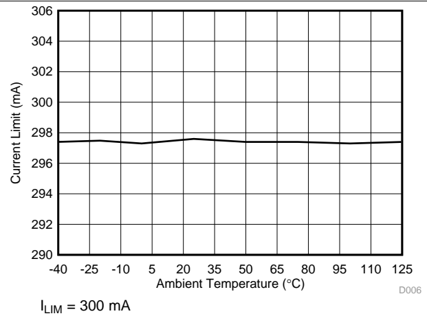
Figure 8. Current Limit vs Ambient Temperature
