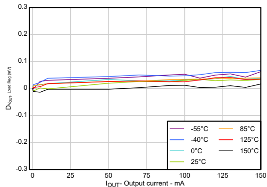
Figure 5-7. Load Regulation
