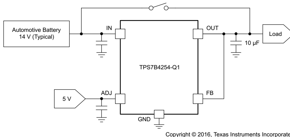
Figure 22. OUT Short to Battery, V_{IN} = V_{BAT}
