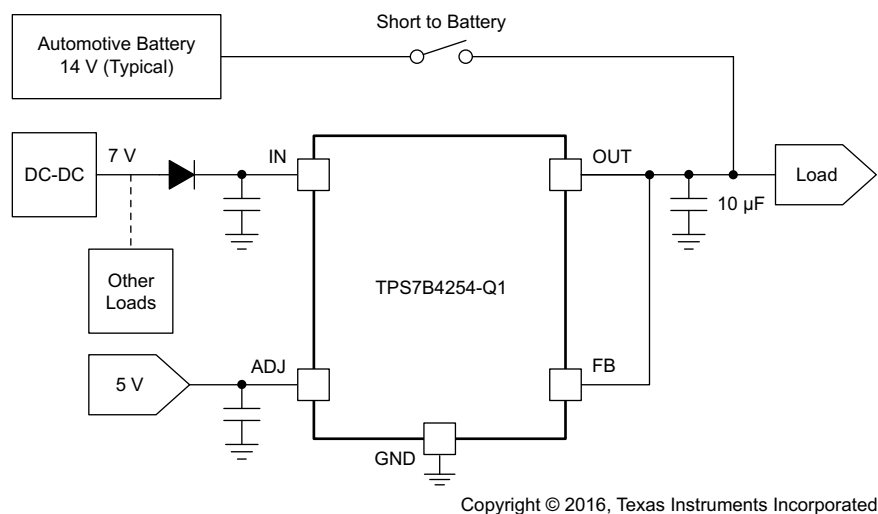
Figure 23. OUT Short to Battery, V_{IN} < V_{BAT}
