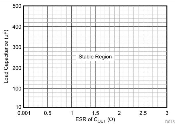
Figure 13. ESR Stability vs Load Capacitance
