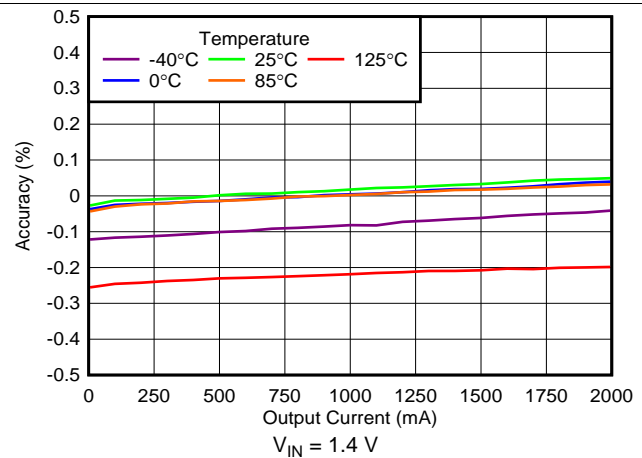
Figure 16. Load Regulation
