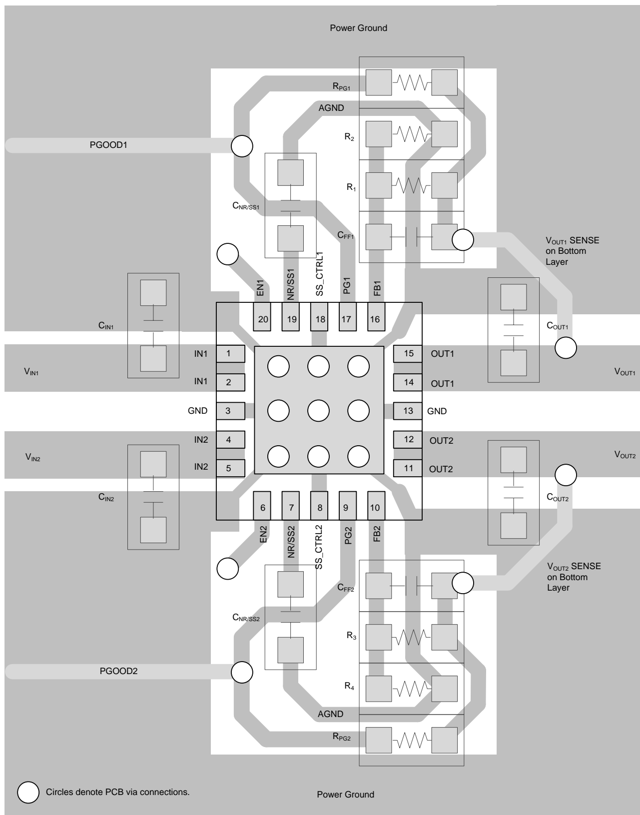
Figure 47. TPS7A88 Example Layout
