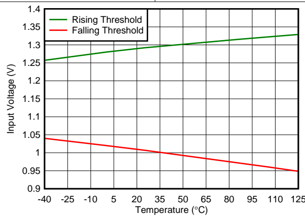
Figure 39. Enable Threshold vs Temperature ( V_{\text{INx}} = 1.4\text{ V} )
