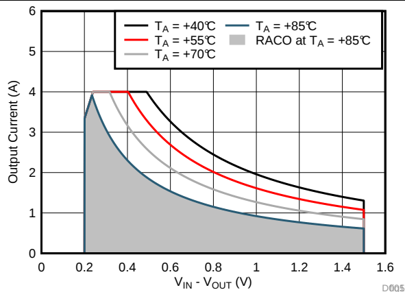
Figure 64. Recommended Area for Continuous Operation for V_{OUT} = 0.9\text{ V}
