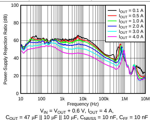
Figure 8. PSRR vs Frequency and I_{OUT} for V_{OUT} = 5\text{ V}
