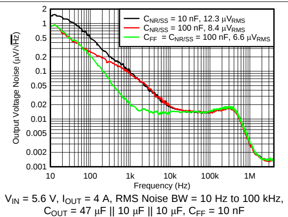
Figure 14. Output Noise vs Frequency and C_{NR/SS}
