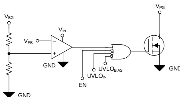
Figure 49. Simplified PG Circuit
