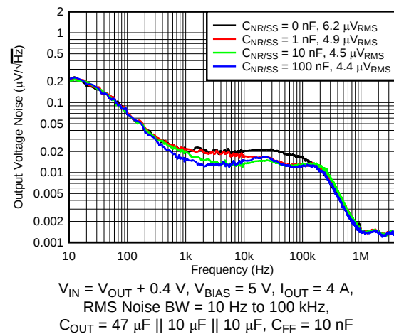
Figure 14. Output Noise vs Frequency and C_{NR/SS}
