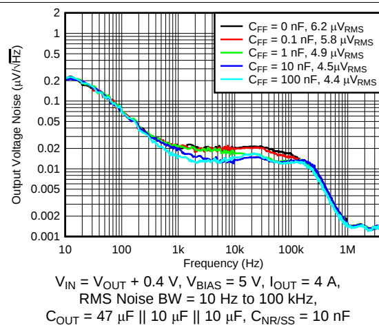
Figure 15. Output Noise vs Frequency and C_{FF}
