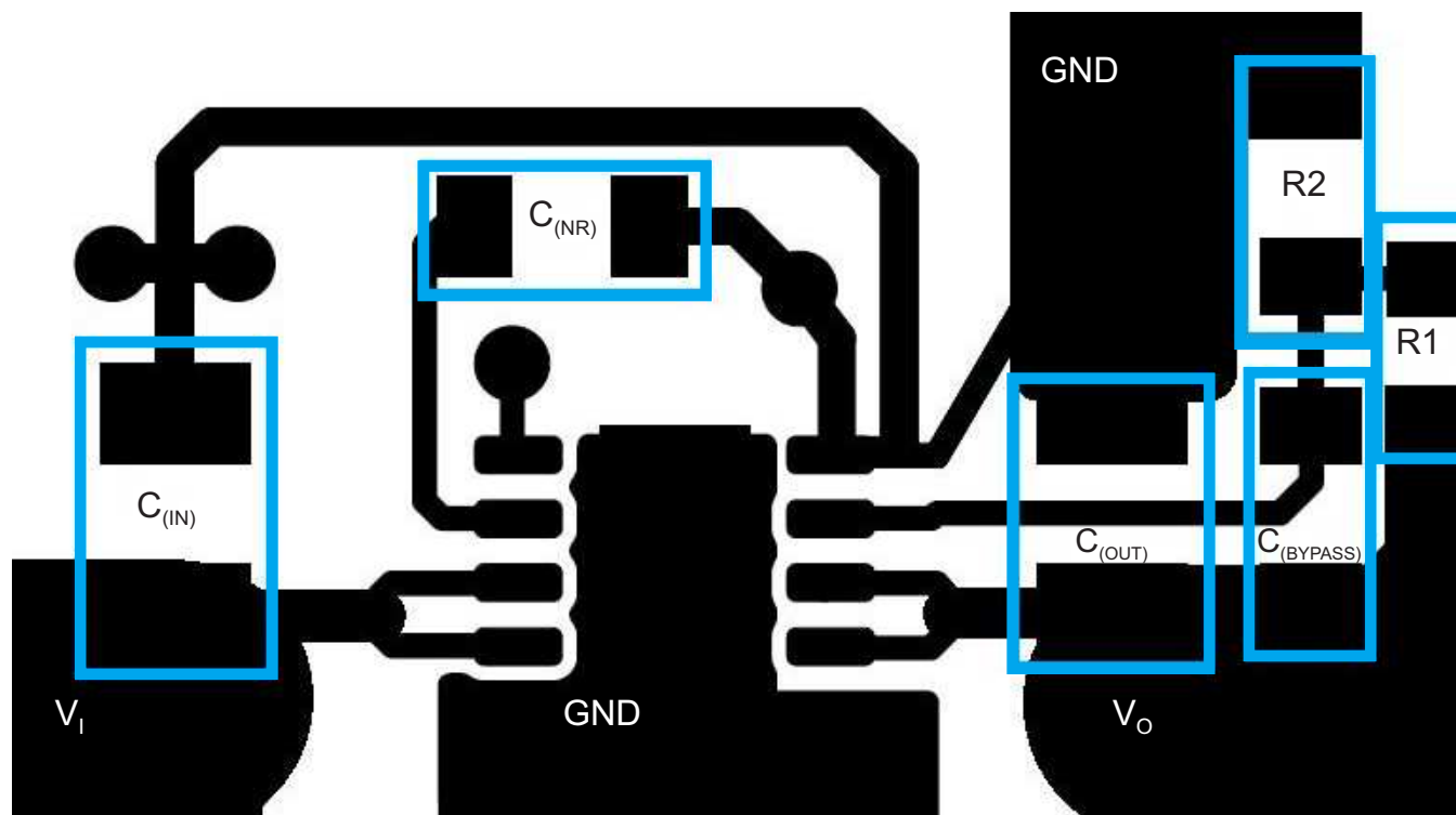
Figure 37. Layout Example
