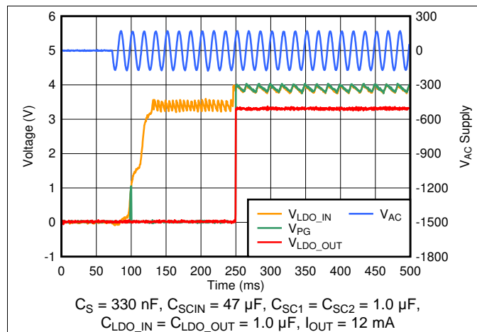
Figure 34. Startup Time
