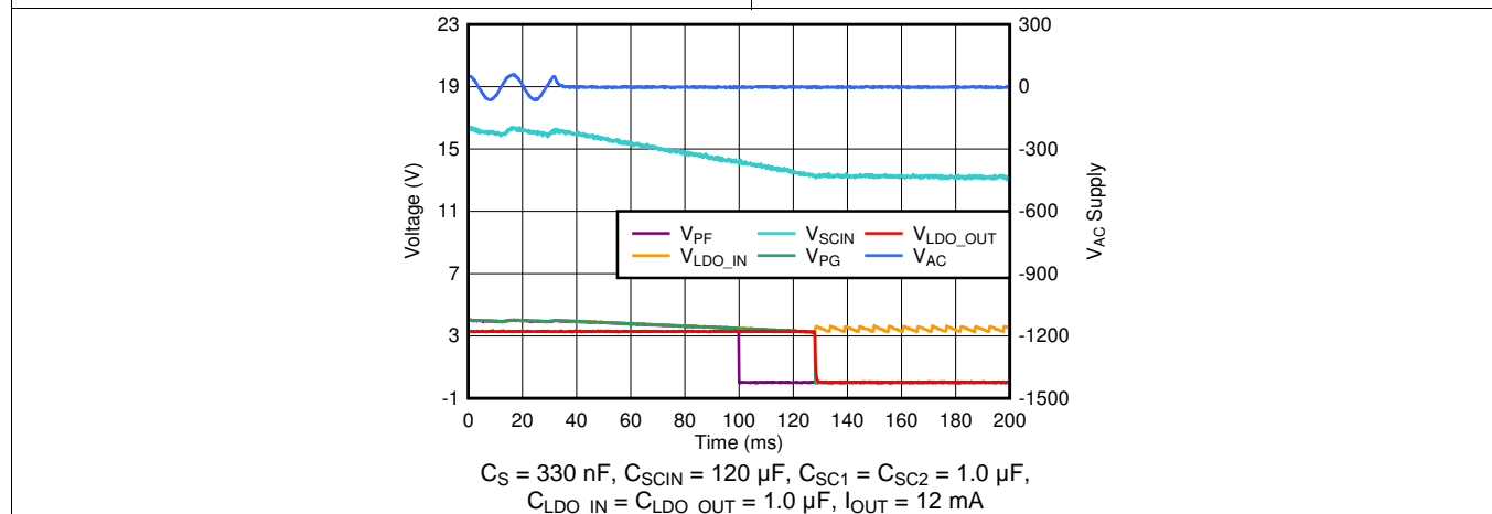
Figure 36. Shutdown Hold-Up Time With a 120- \mu F C_{SCIN} Capacitor
