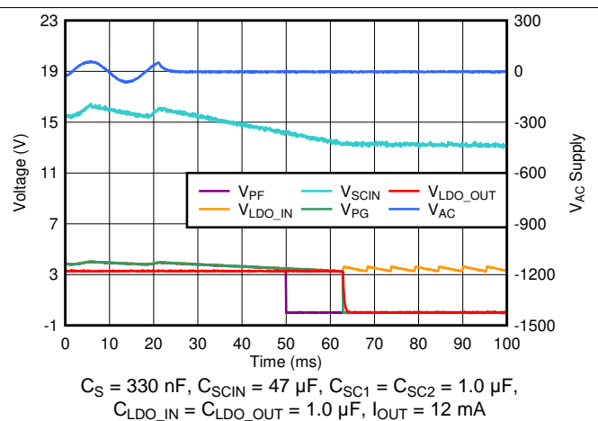
Figure 35. Shutdown Hold-Up Time With a 47- \mu F C_{SCIN} Capacitor
