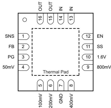
Figure 4-1. RGT Package, 16-Pin With Exposed Thermal Pad (Top View)
