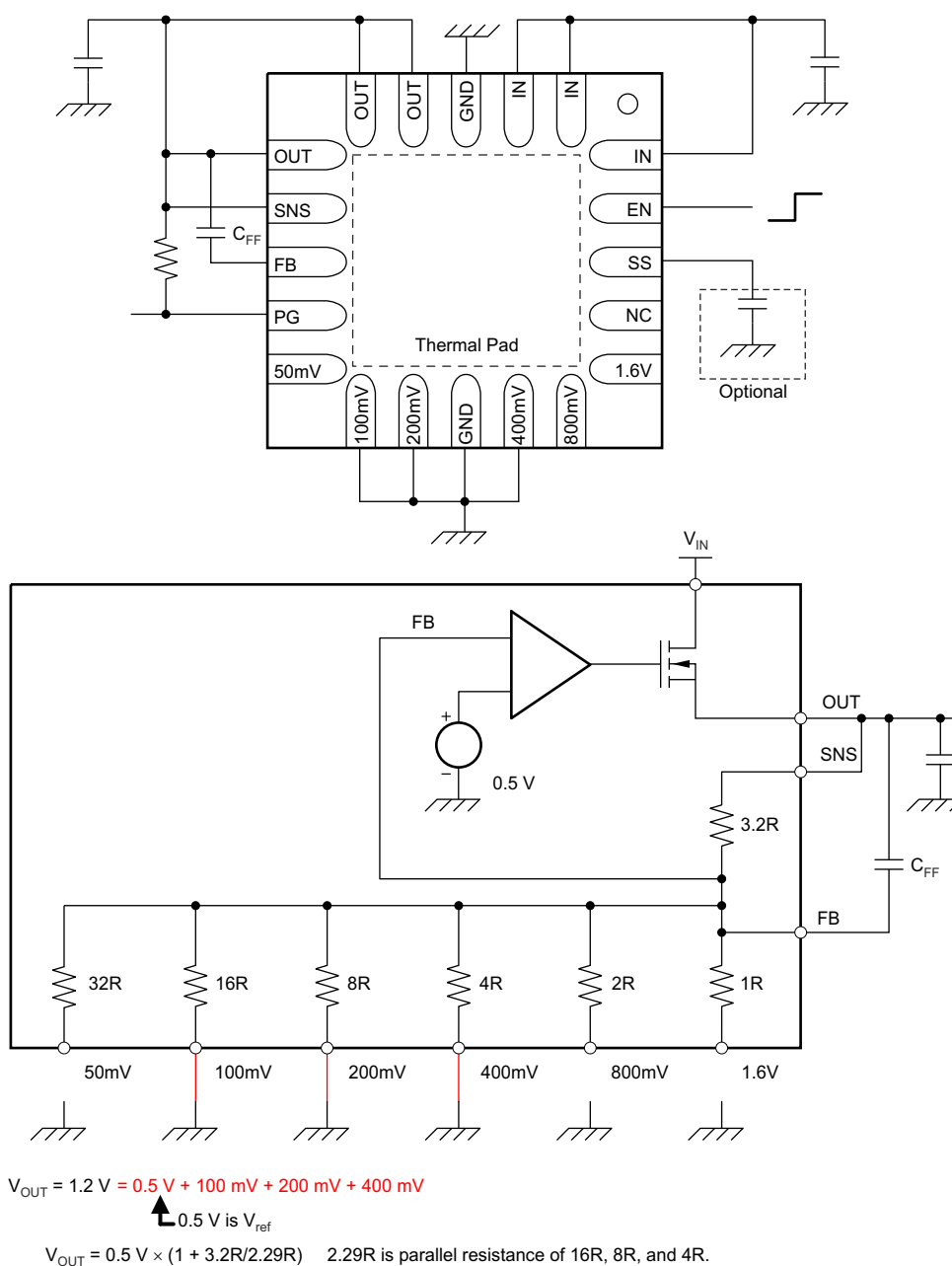
Figure 6-2. 1.2-V Configuration
