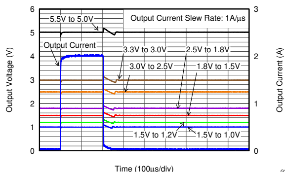
Load Transient Response With Seven Different Outputs
