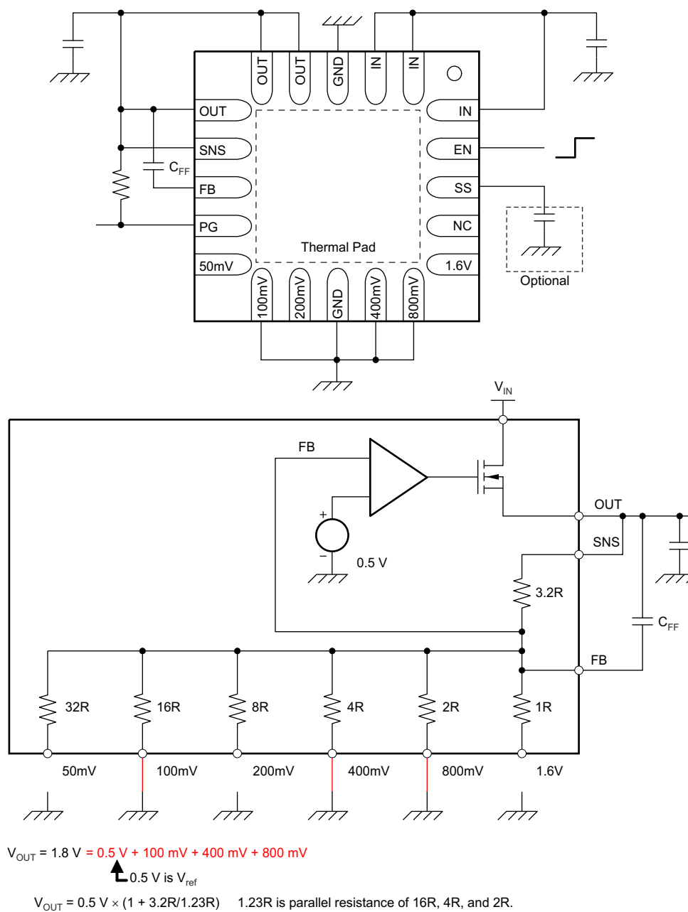
Figure 6-3. 1.8-V Configuration
