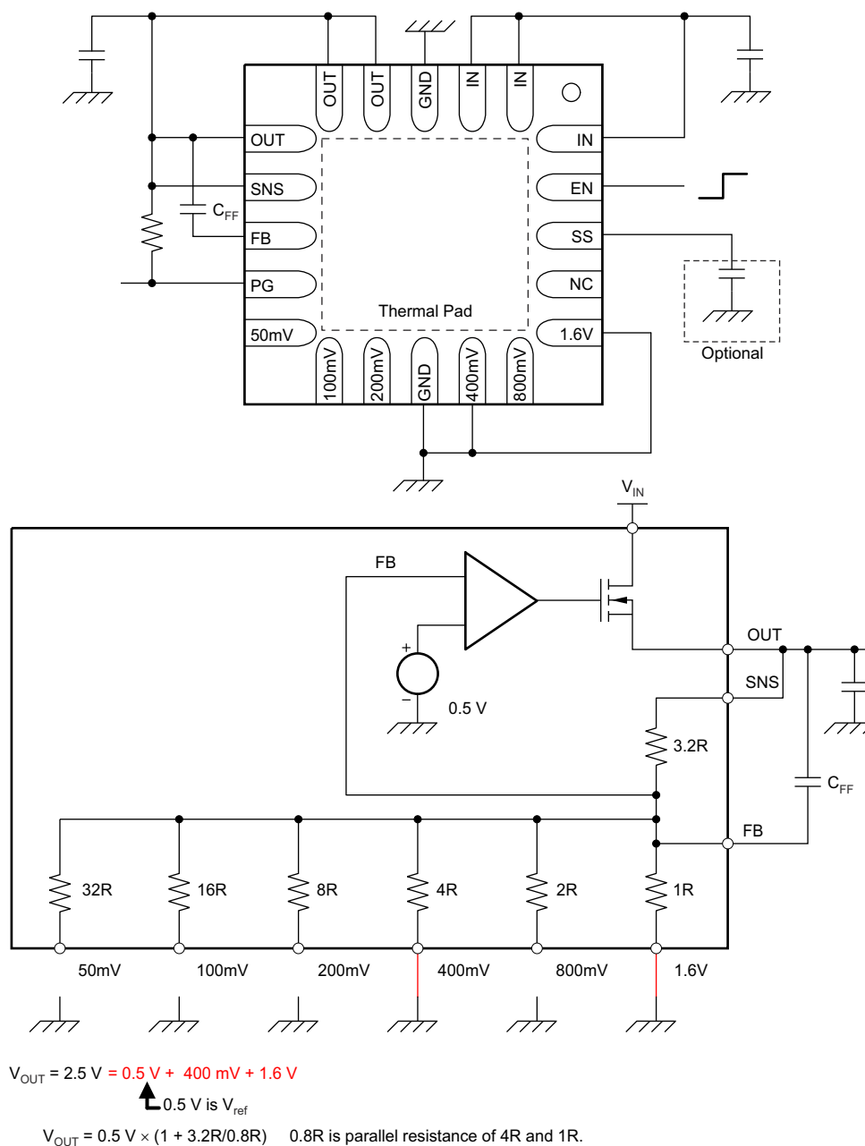
Figure 6-4. 2.5-V Configuration
