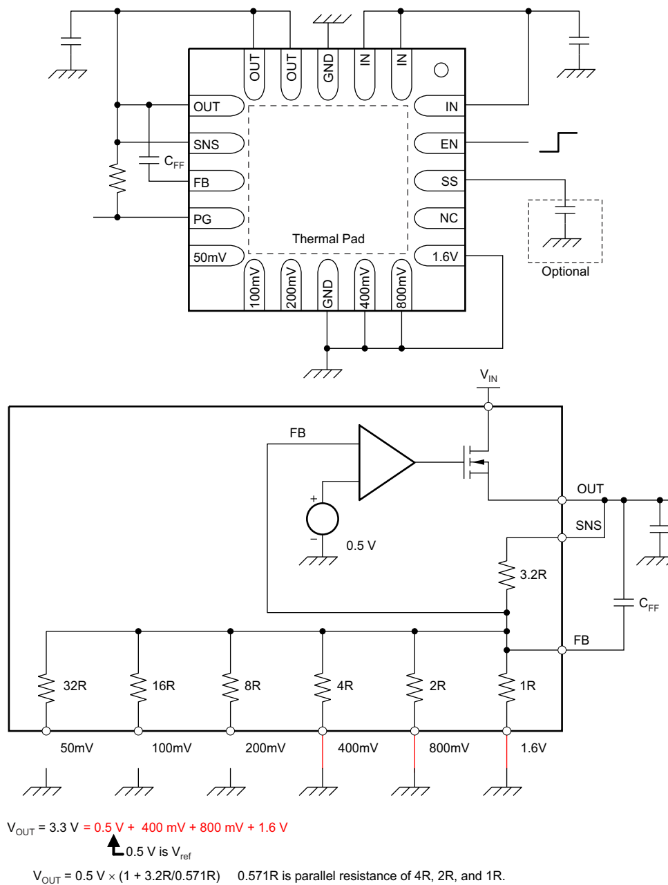
Figure 6-5. 3.3-V Configuration
