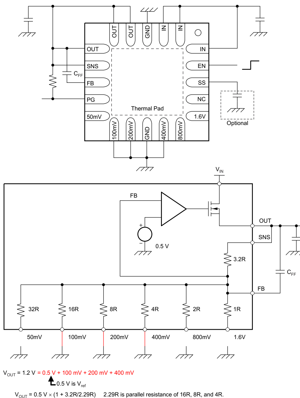
Figure 6-2. 1.2-V Configuration
