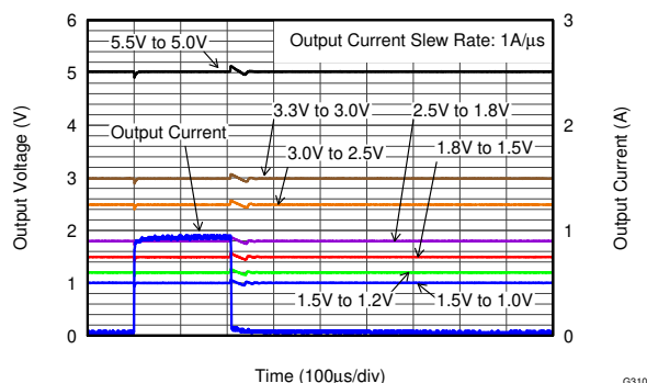
Load Transient Response With Seven Different Outputs: 1.5 V IN to 1 V OUT , 1.5 V IN to 1.2 V OUT , 1.8 V IN to 1.5 V OUT , 2.5 V IN to 1.8 V OUT , 3 V IN to 2.5 V OUT , 3.3 V IN to 3 V OUT , and 5.5 V IN to 5 V OUT
