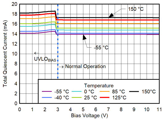
Figure 6-169. Total Quiescent Current vs V_{BIAS} for V_{OUT} = 0.5 V, V_{IN} = 1.1 V, CP Enabled, I_{OUT} = 0 A
