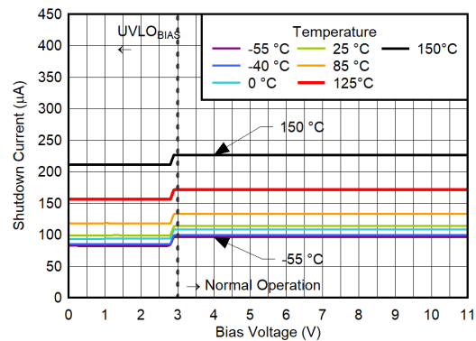
Figure 6-206. IN Pin Shutdown Current vs V_{BIAS} for V_{IN} = 6 V, V_{OUT(nom)} = 0.5 V, CP Disabled
