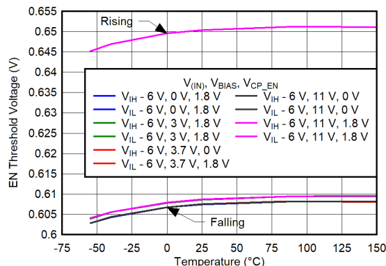
Figure 6-209. EN Threshold Voltage vs Temperature for V_{IN} = 6 V, V_{OUT} = 0.5 V
