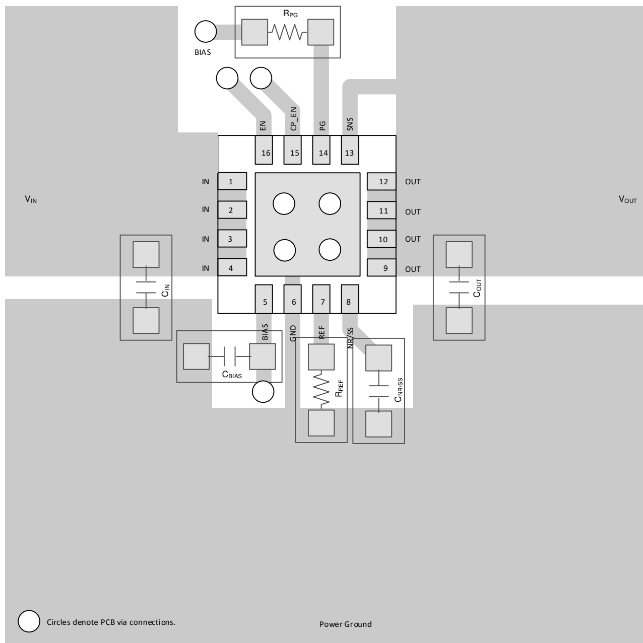
Figure 8-44. Recommended Layout
