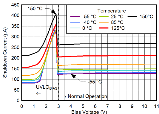
Figure 6-205. BIAS Pin Shutdown Current vs V_{BIAS} for V_{IN} = 6 V, V_{OUT(nom)} = 0.5 V, CP Disabled
