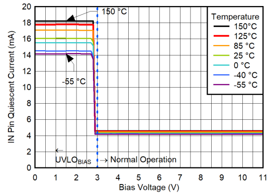
Figure 6-170. IN Pin Quiescent Current vs Bias Voltage for V_{OUT} = 0.5 V, V_{IN} = 1.1 V, CP Enabled, I_{OUT} = 0 A
