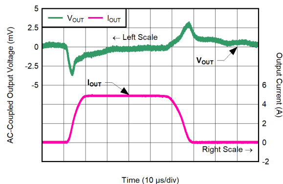
Figure 6-44. Load Transient for V_{OUT} = 5.2 V, I_{OUT} = 100 mA to 5 A, CP Disabled, SR = 1 A/ \mu s, V_{BIAS} = 8.4 V
