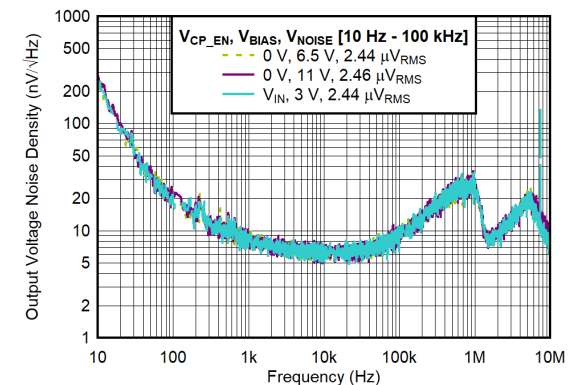
Figure 6-24. Output Voltage Noise Density vs Frequency and V_{CP\_EN} for V_{OUT} = 3.3 V
