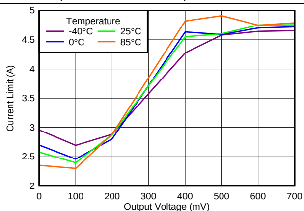
Figure 38. Foldback Current Limit vs Temperature
