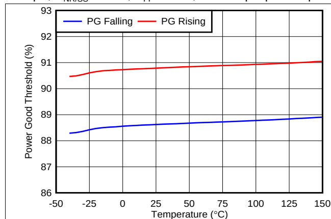
Figure 37. PG Threshold vs Temperature
