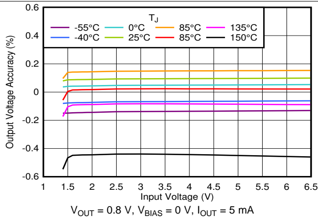
Figure 27. Line Regulation Without Bias
