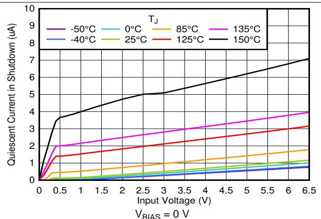
Figure 30. Shutdown Current vs Input Voltage
