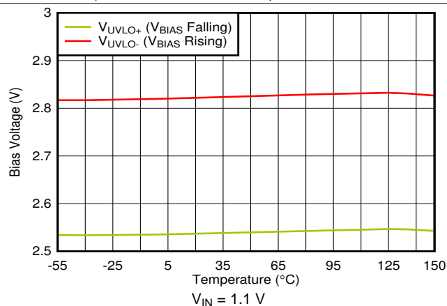
Figure 20. V_{BIAS} UVLO vs Temperature
