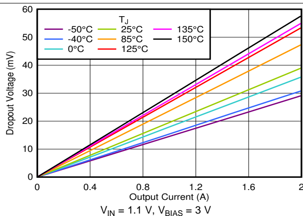
Figure 10. Dropout Voltage vs Output Current With Bias
