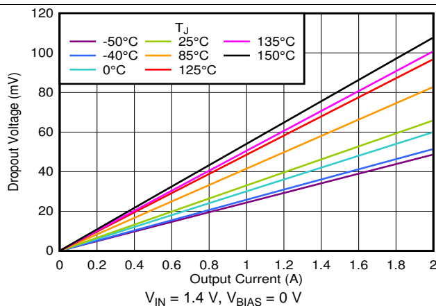
Figure 9. Dropout Voltage vs Output Current Without Bias
