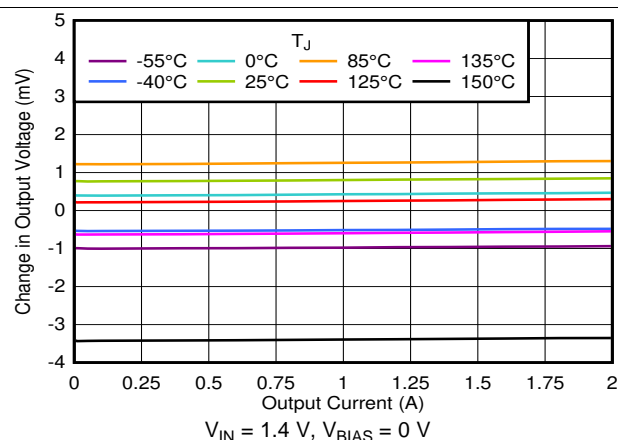
Figure 12. Load Regulation With Bias
