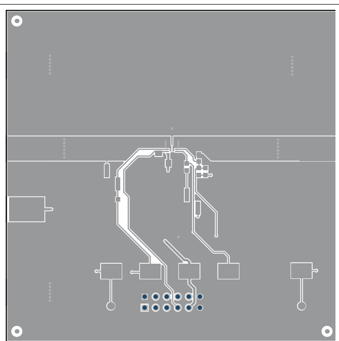
Figure 35. Top Layer Routing
