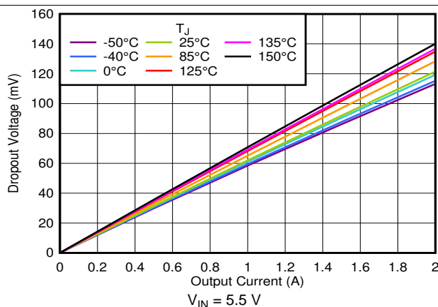
Figure 11. Dropout Voltage vs Output Current (High V_{IN} )
