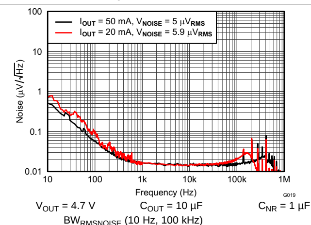
Figure 22. Noise vs Output Current
