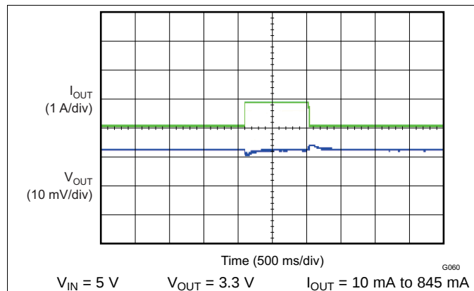
Figure 19. Load Transient
