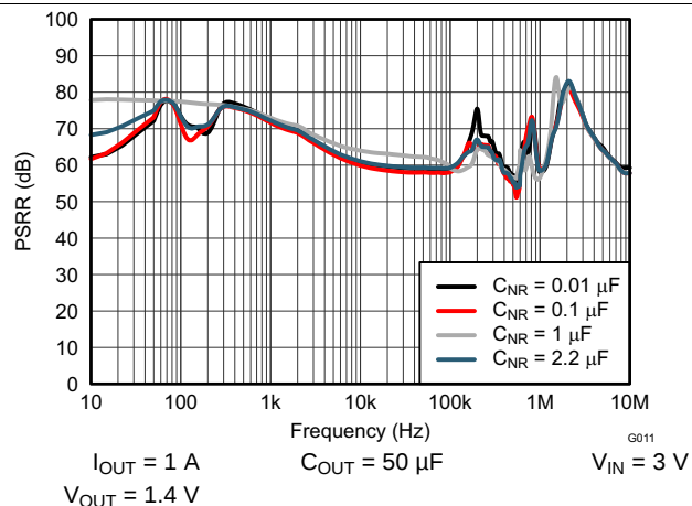
Figure 11. Power-Supply Rejection Ratio vs C_{\text{NR}}
