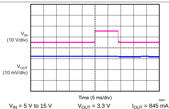
Figure 20. Line Transient
