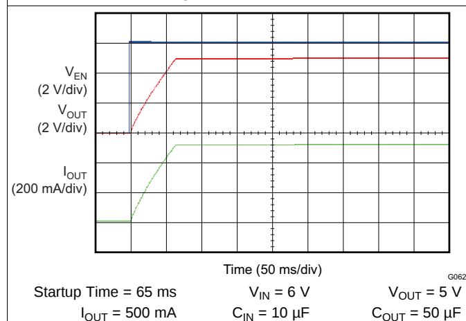
Figure 21. Startup
